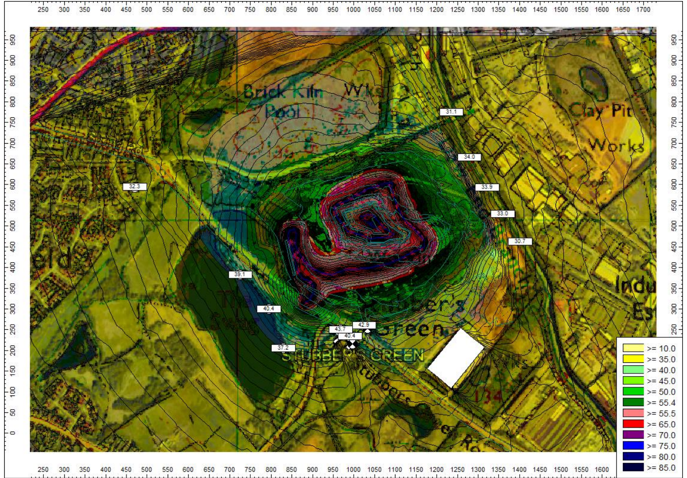
NOISE MAP 6-1: NOISE CONTOURS FOR FINAL EXTRACTION (YEARS 1 TO 3)
