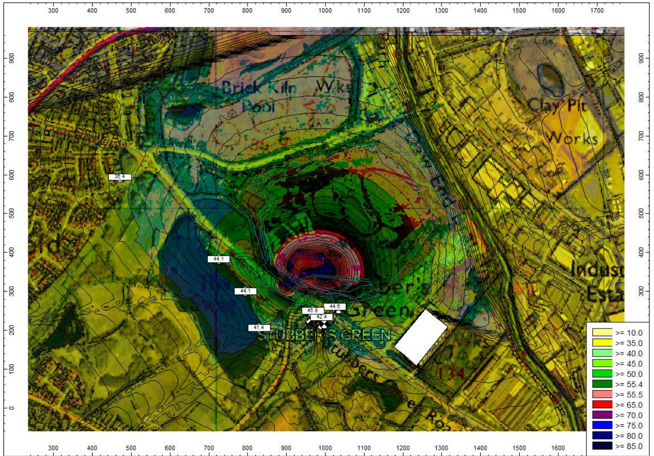
NOISE MAP 6-10: NOISE CONTOURS FOR YEARS 15 TO 18 WITH MITIGATION
