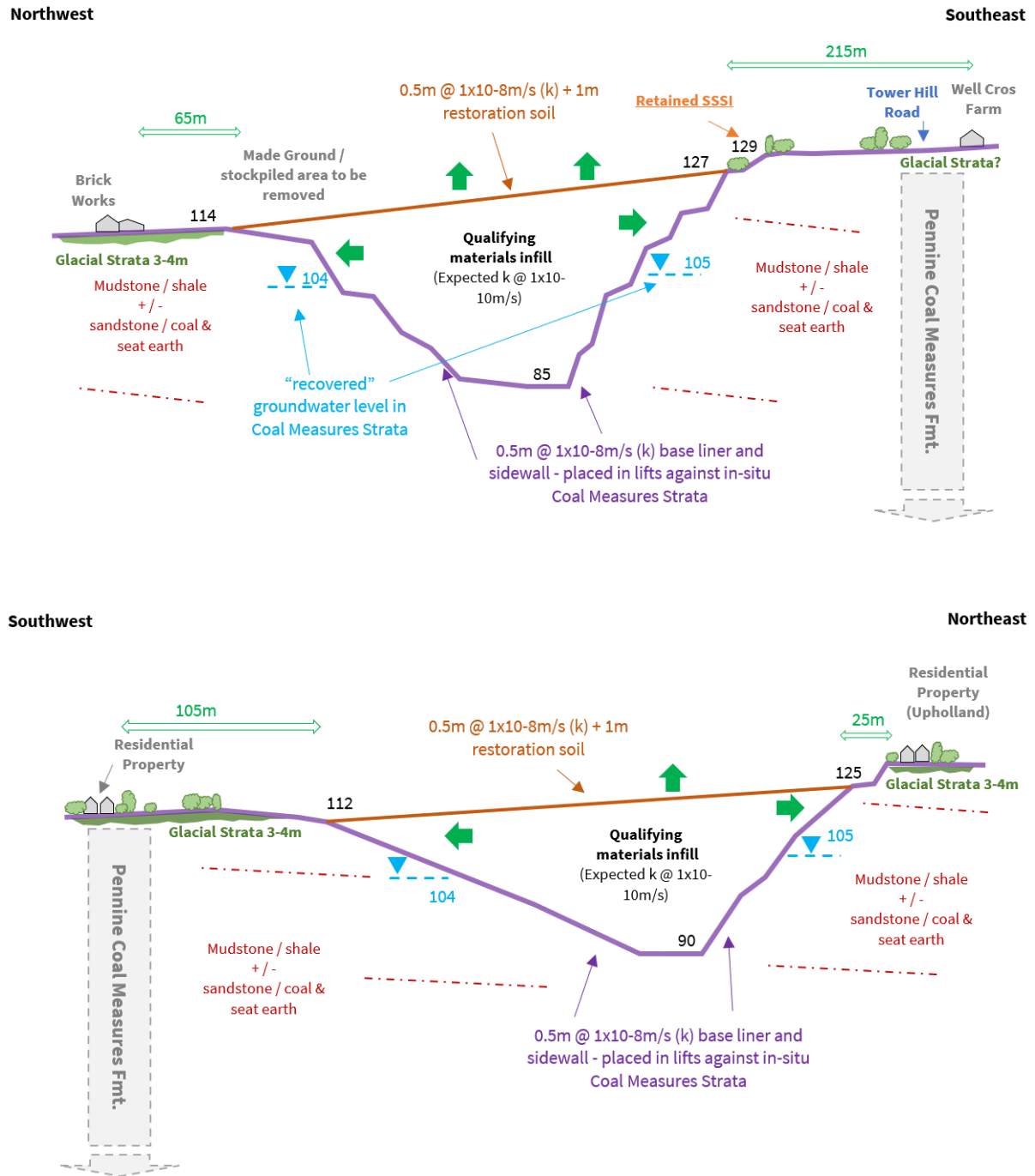
Figure 2 Schematic Conceptual Site Model
