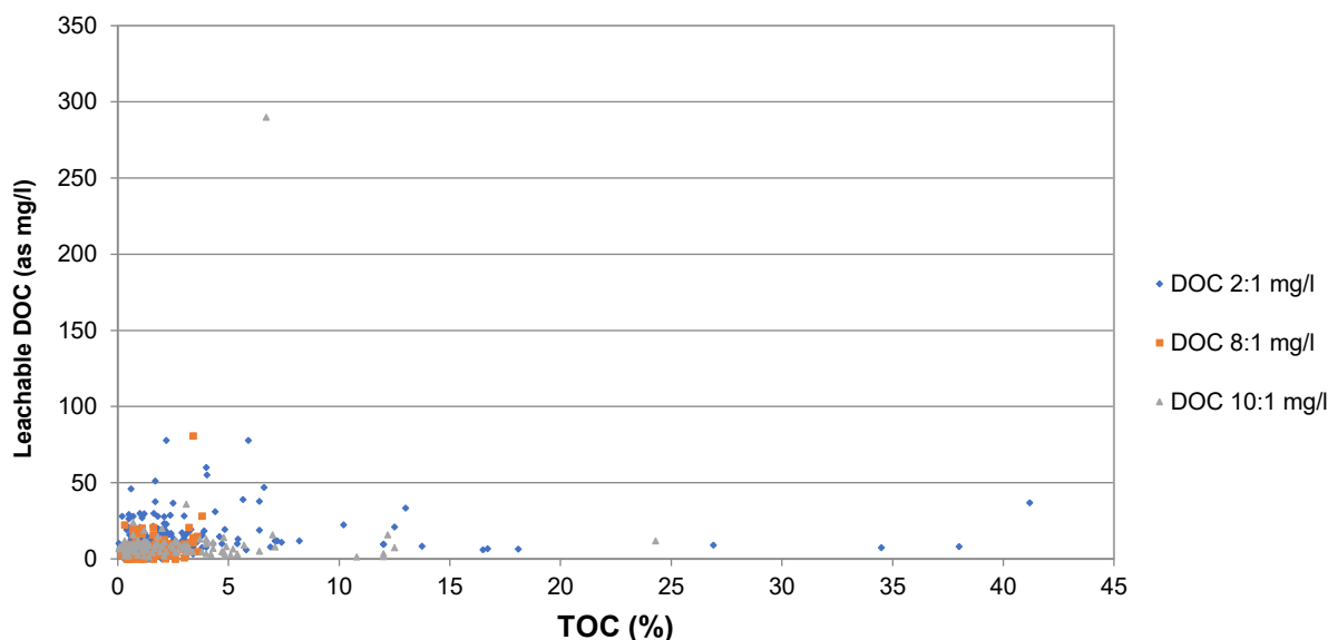
Figure 5 Leachability of DOC in relation to TOC
