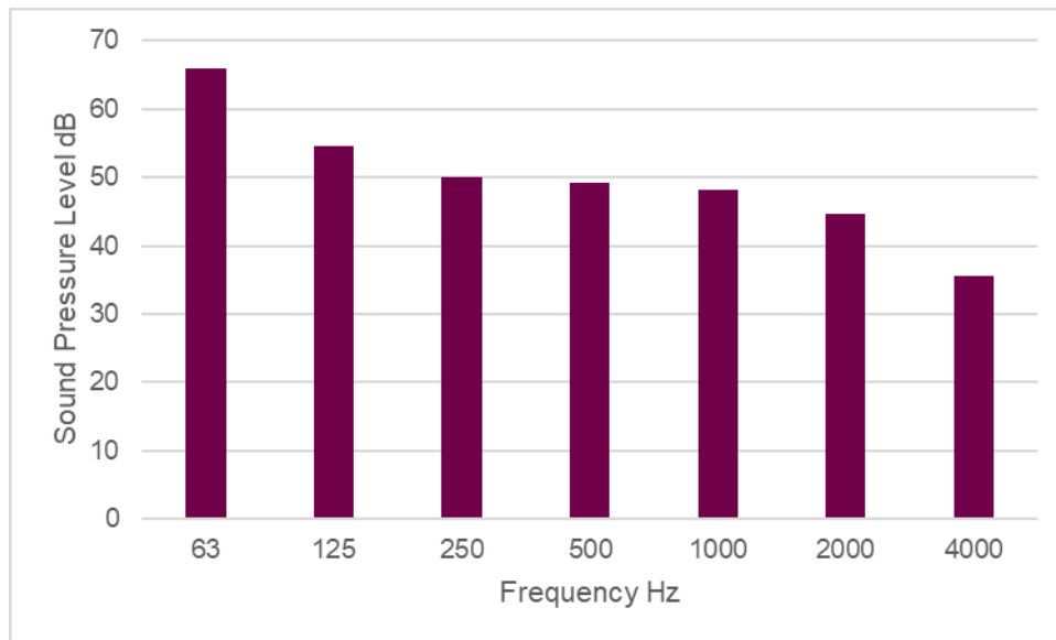
Figure 4: Linear Octave Band Spectrum
