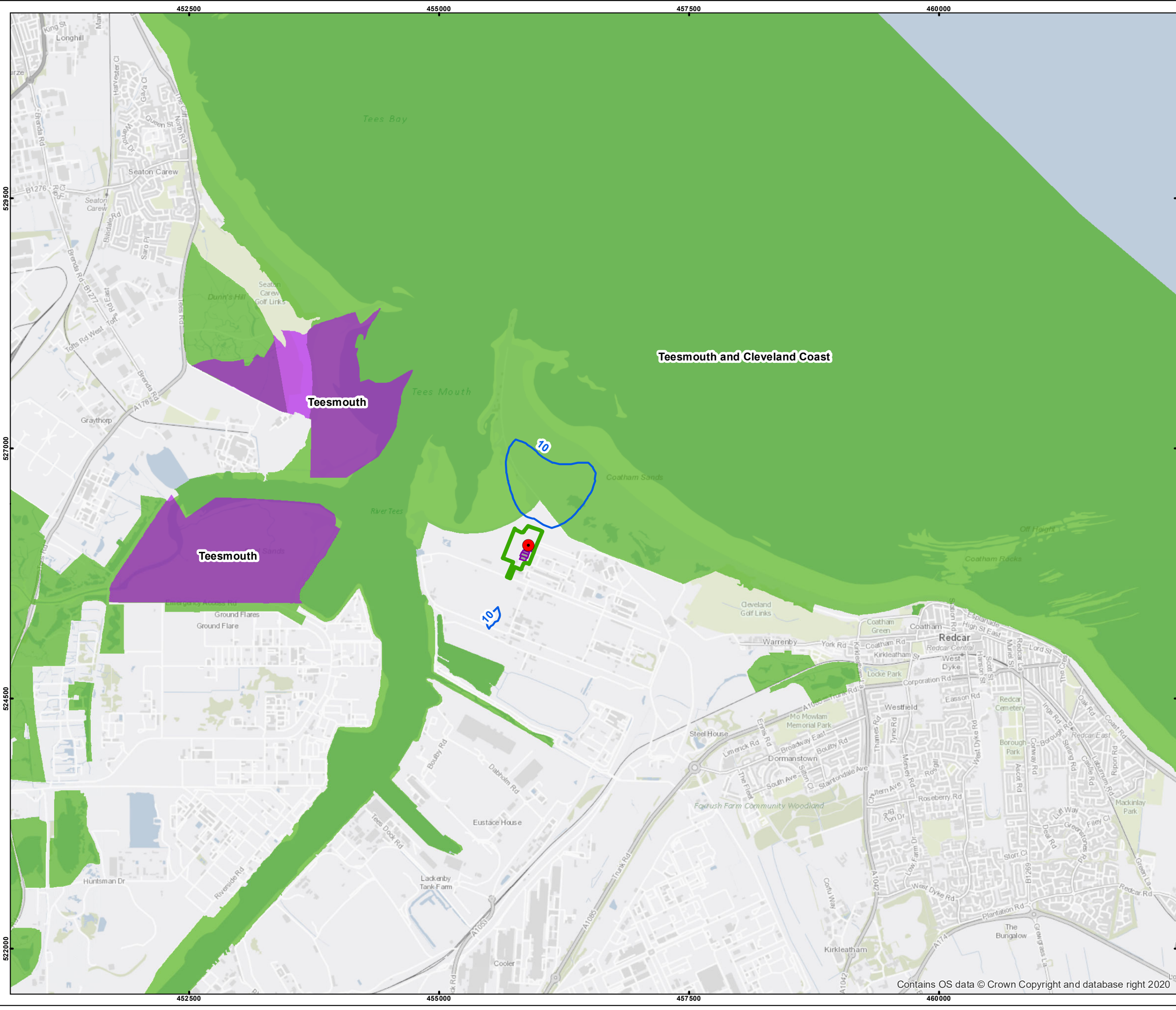
Figure 18: Daily Mean Oxides of Nitrogen
