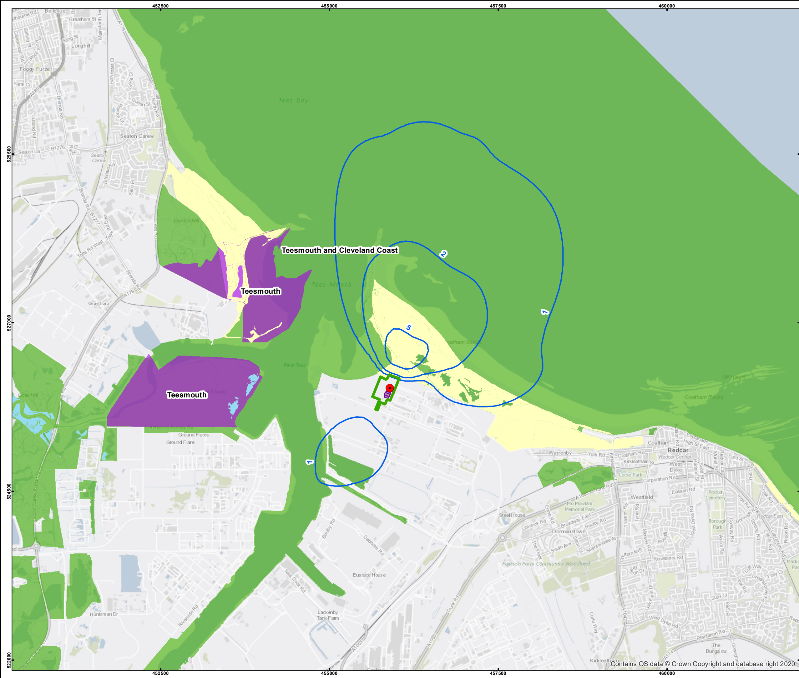
Figure 17: Annual Mean Oxides of Nitrogen
