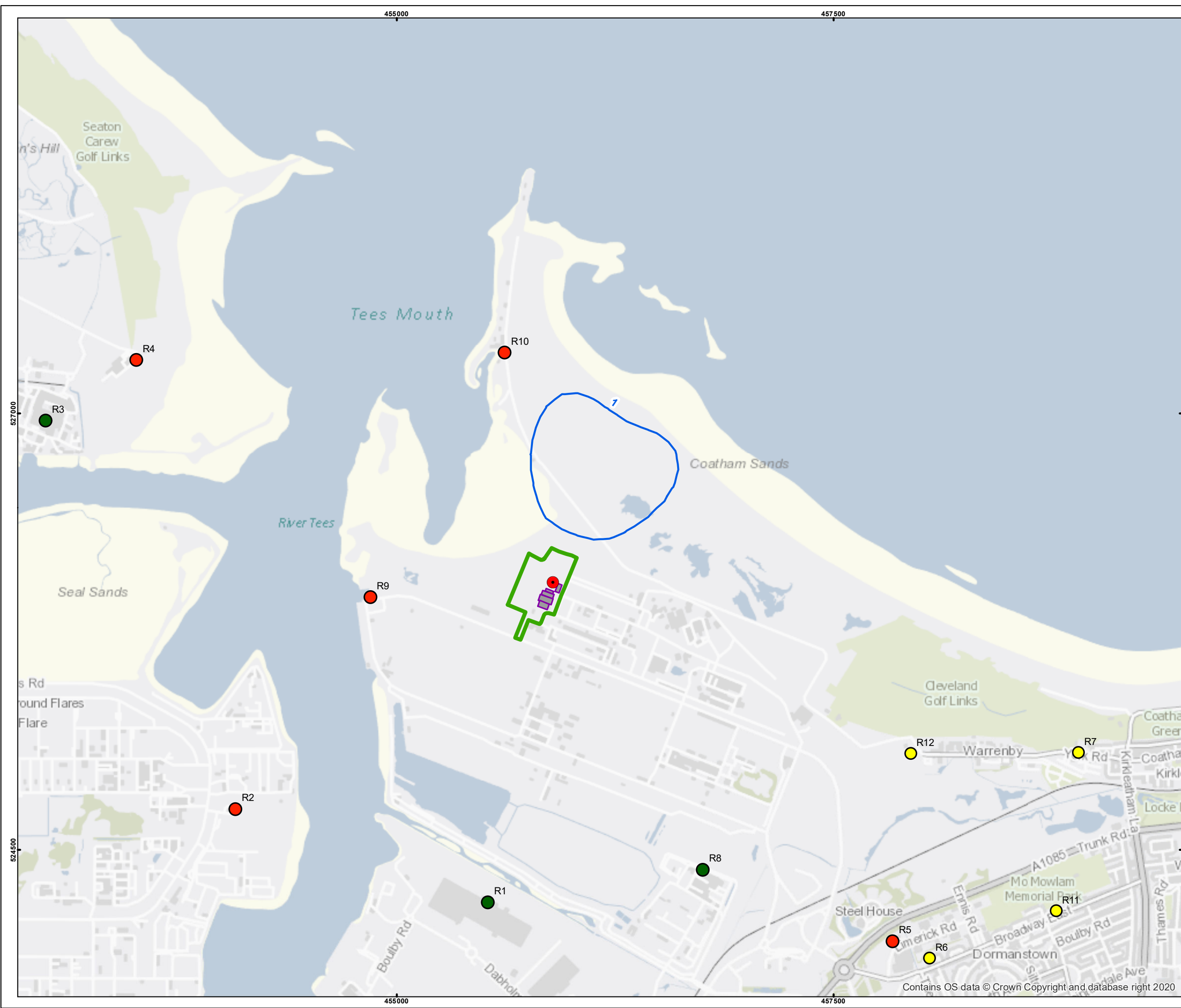
Figure 13: Annual Mean PAHs as Benzo[a]pyrene
