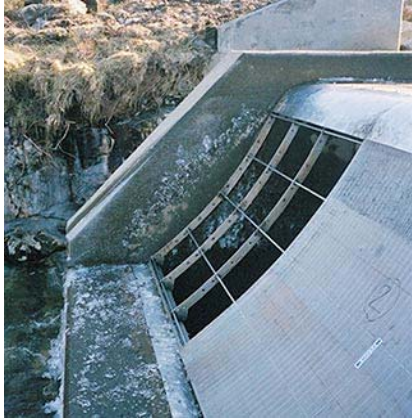
Plate 3.5 Example of a Screen A Coanda installation (Dulas Hydro)
