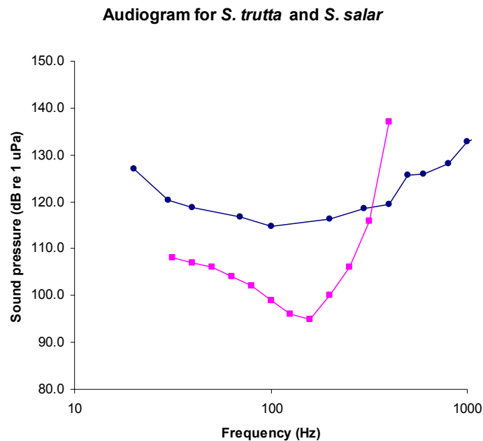
Figure 3.15 Audiograms of Atlantic salmon ( Salmo salar ) (■) and trout ( S. trutta ) (●) (Nedwell et al. , 2003).
