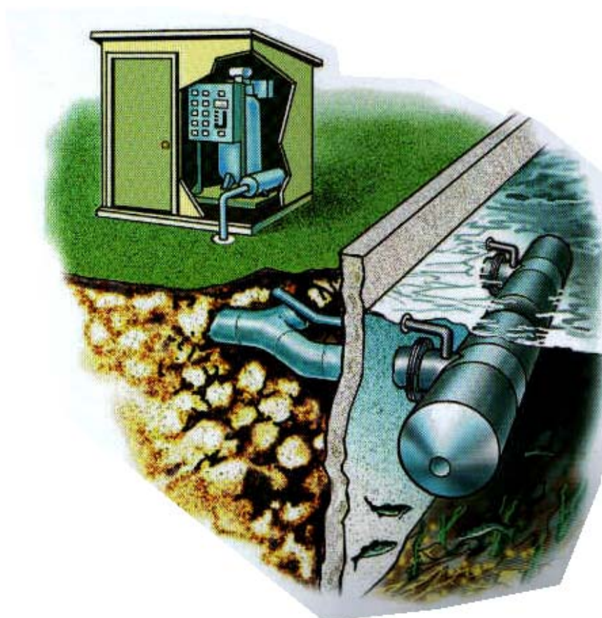
Figure 3.8 Illustration of bulkhead mounted PWWC screen array with manifold and air backwash system; the compressor is located in a bankside hut but could be located in any neighbouring building. (courtesy Johnson Screens)
