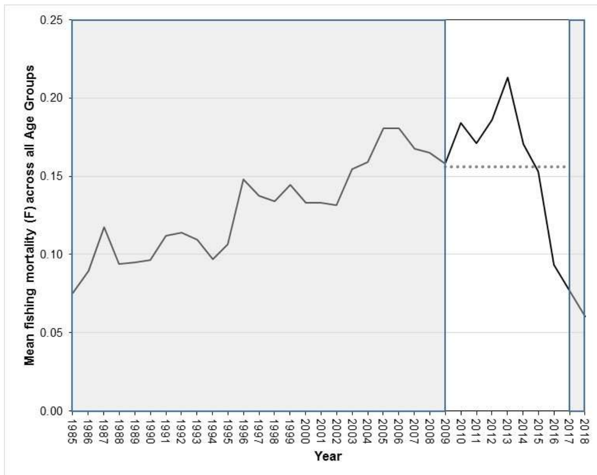
Figure 1. Mean fishing mortality (F) across all Age Groups of seabass for the years 1985 to 2018 ( — ) together with the mean value of F across all Age Groups for the years 2009 – 2017 ( ..... ) coinciding with the period of the Comprehensive Impingement Monitoring Programme at SZB. Data from ICES (2019).
