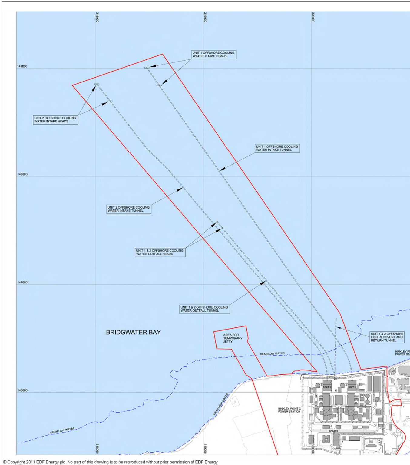
Figure B1: Intake, outfall and fish recovery and return (FRR) system tunnel alignments and head locations
