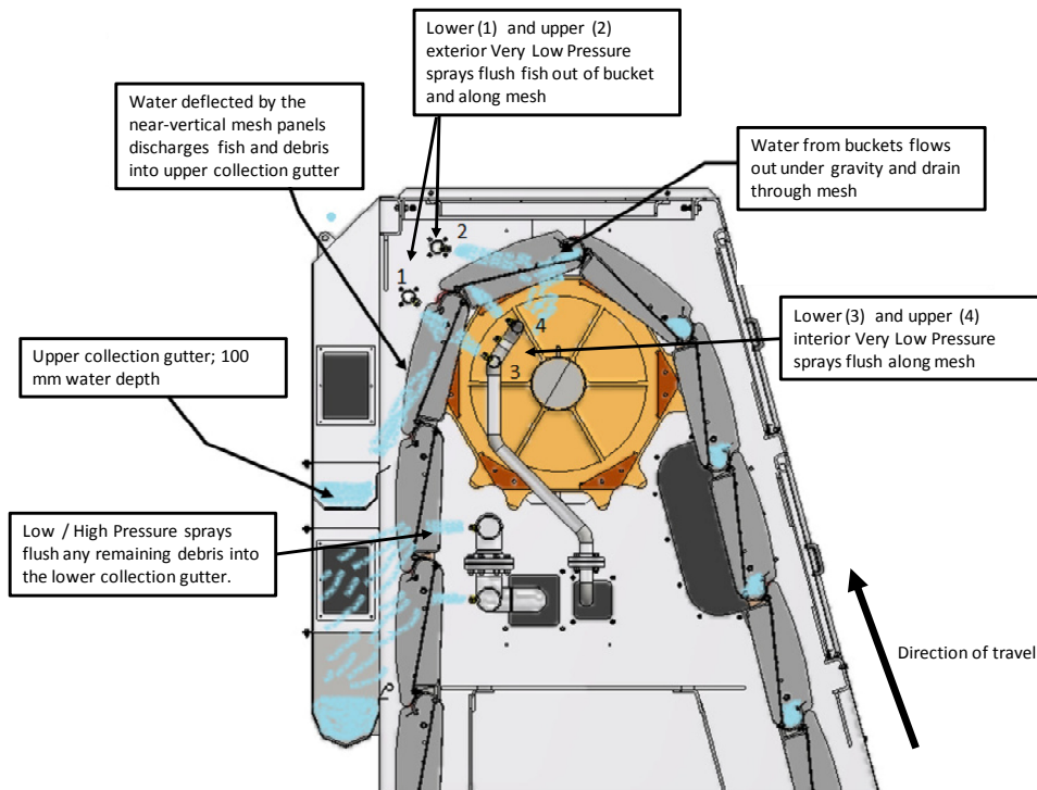
Figure 18: Detailed section of band screen head frame showing flushing and discharge of collected material.
