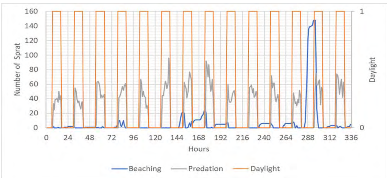
Figure 8: Instantaneous number of beached (blue) and eaten (grey) particles, overlaying daylight hours (orange).
