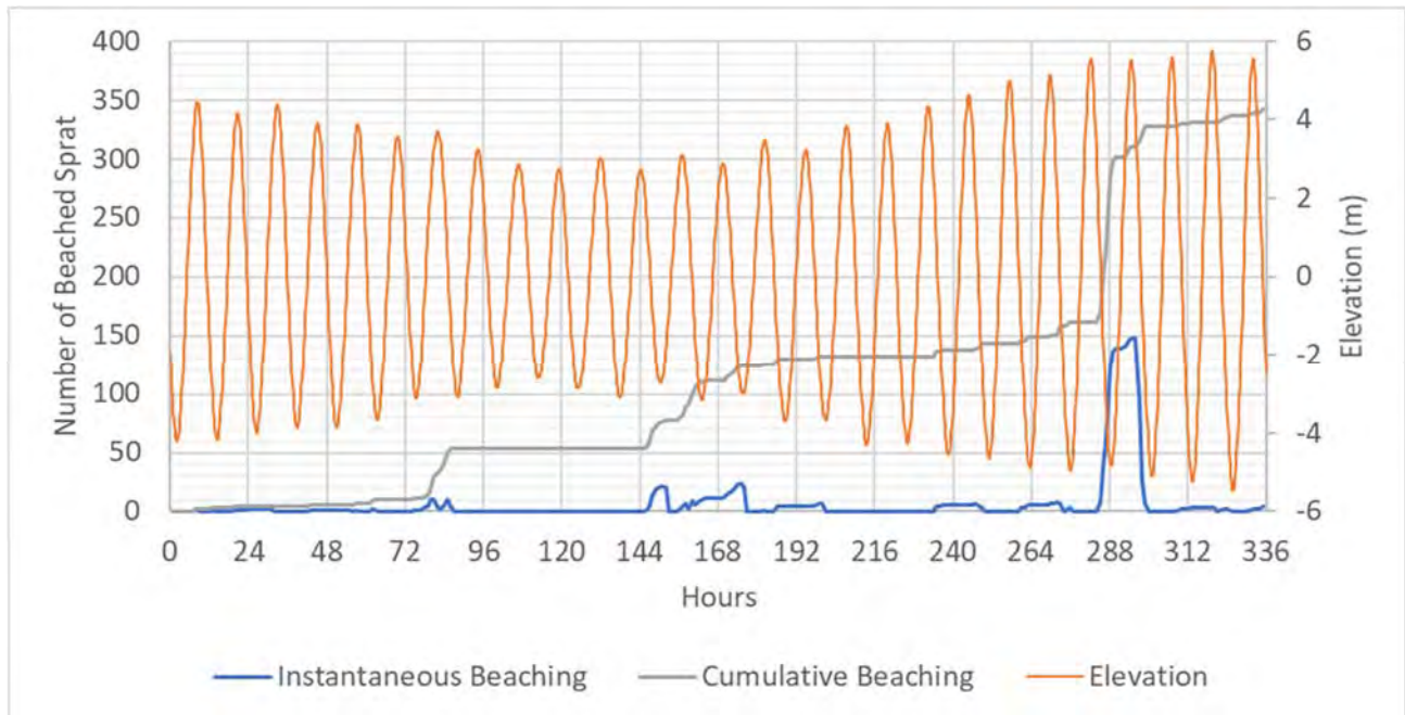
Figure 7: Instantaneous (blue) and cumulative number of beached particles (grey) over the 14-day simulation, with the free surface elevations at Hinkley Point (orange).
