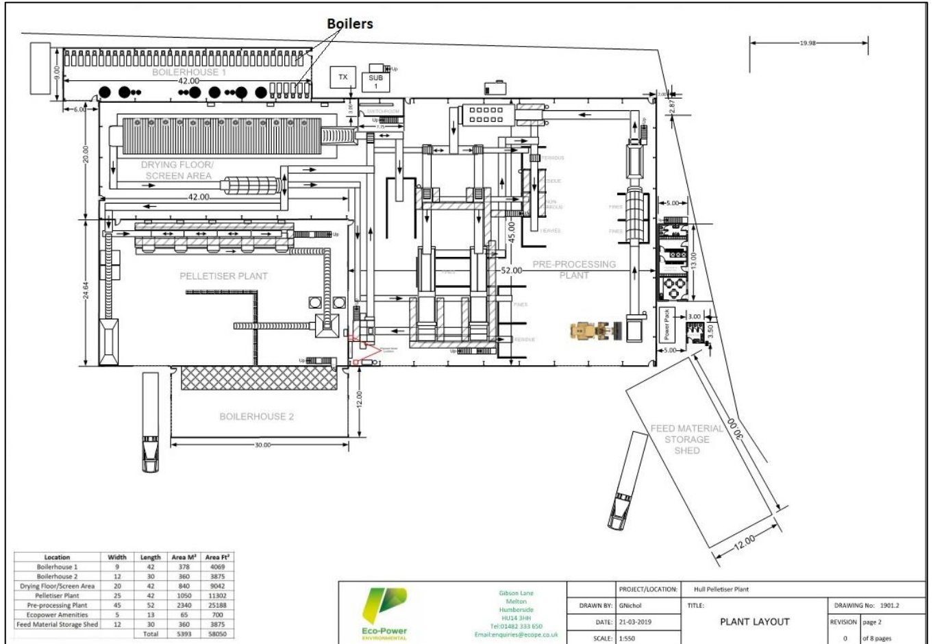
Figure 1-3. Site Layout
