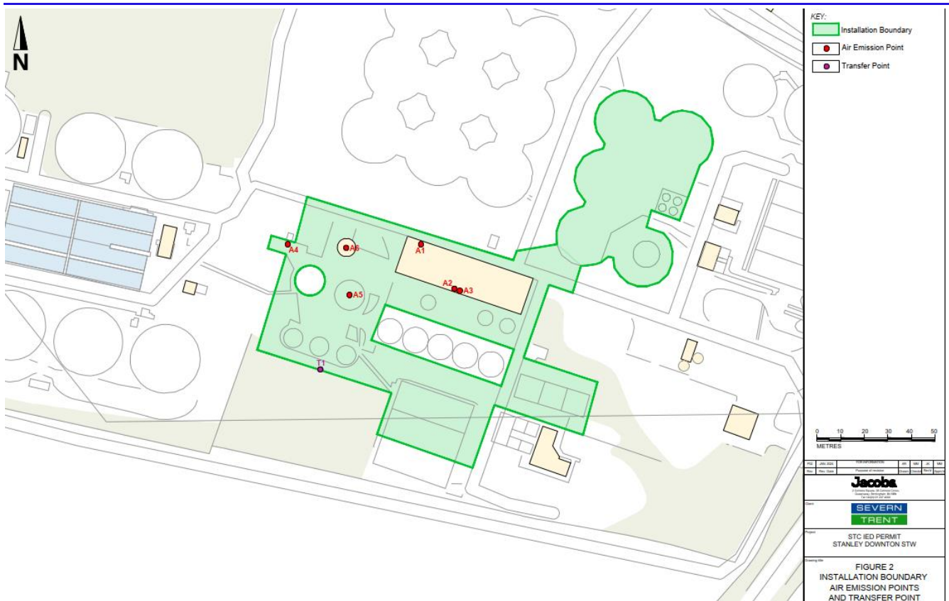
Figure 1.1 Boundary of the permitted IED area and the assets contained in Stanley Downton STW
