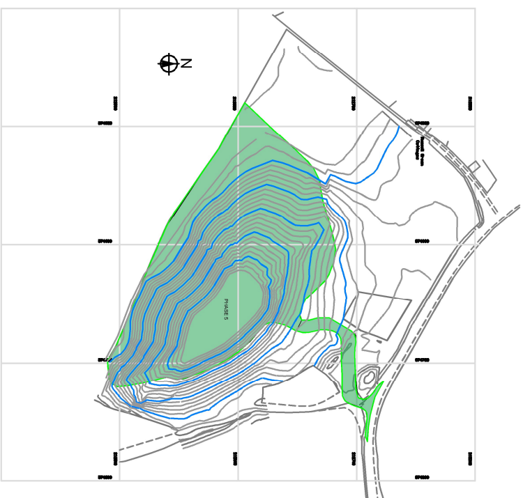
PHASE 5 Whole site landscaping Removal of Site Infrastructure
