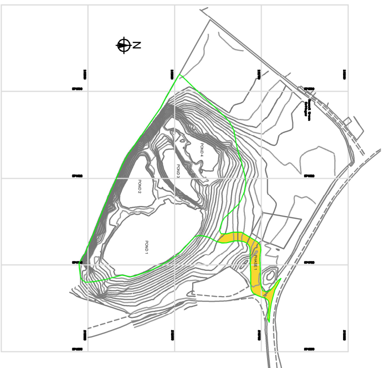
PHASE 1 Construction of site entrance, internal haul road to working area, and compound. Install site office, wheel wash and bunded fuel tank.
