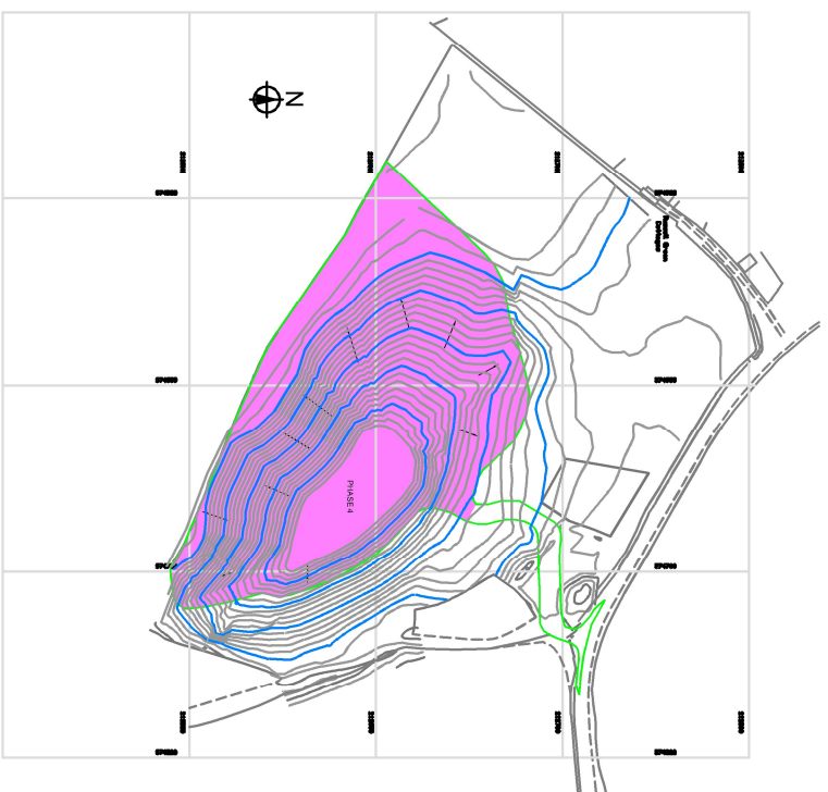
PHASE 4 Stabilise quarry face. Key-in trenching against slopes, in 250mm horizontal compacted layers from base. Creation of new pond.
