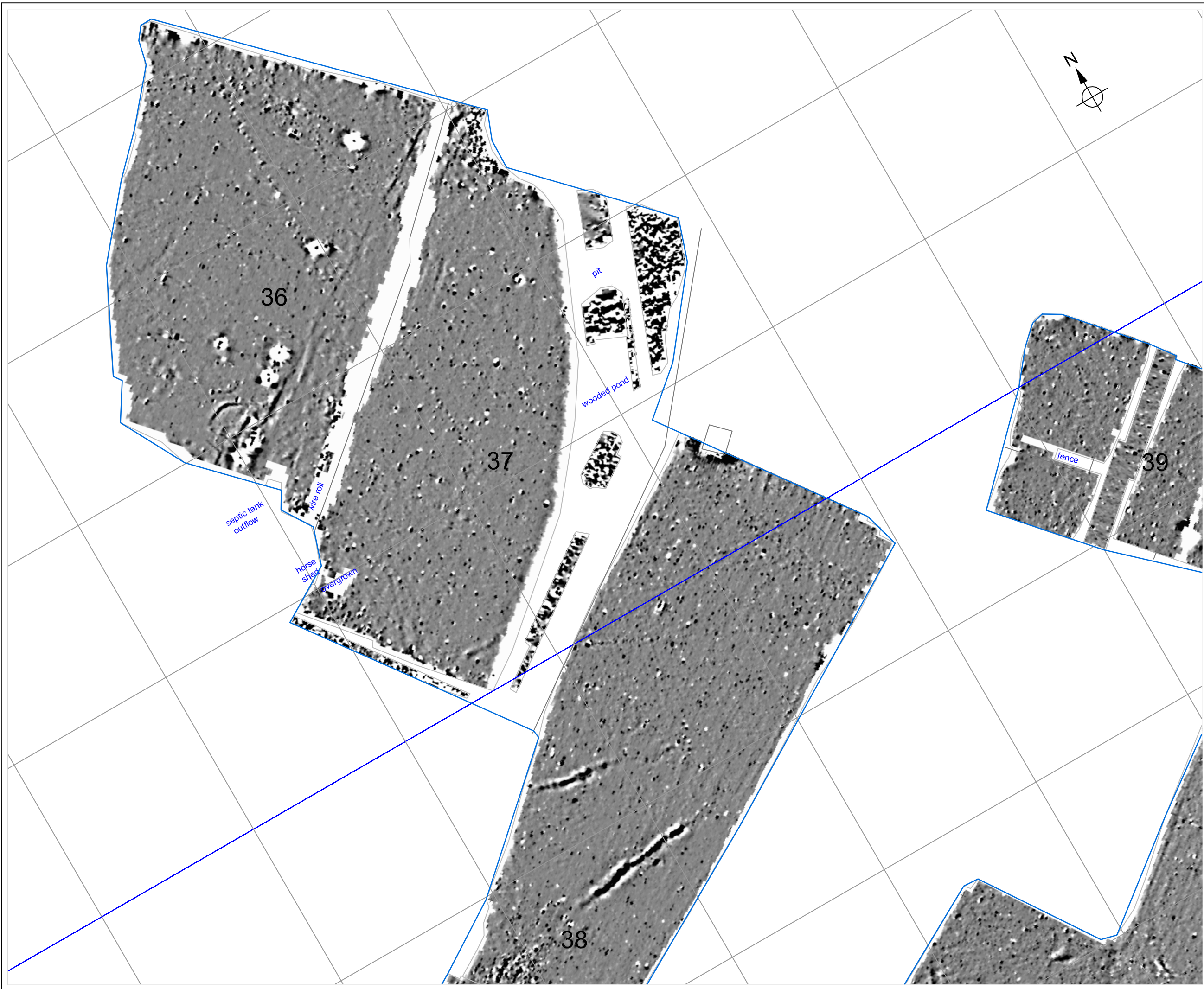
Figure 35 Magnetometer survey: grey scale plot (9/11) [Chilswell Valley survey]
