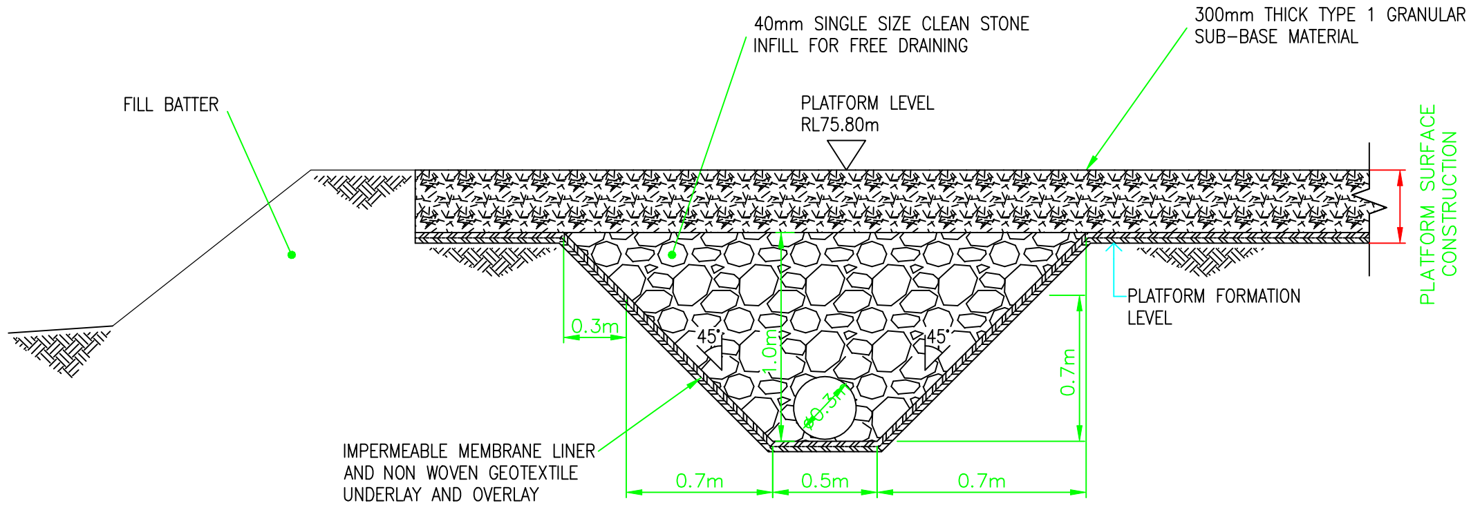
INDICATIVE SECTION THROUGH COVERED DITCH CONSTRUCTION RETENTION AND WELL ABANDONMENT PHASES (1:25 SCALE)
