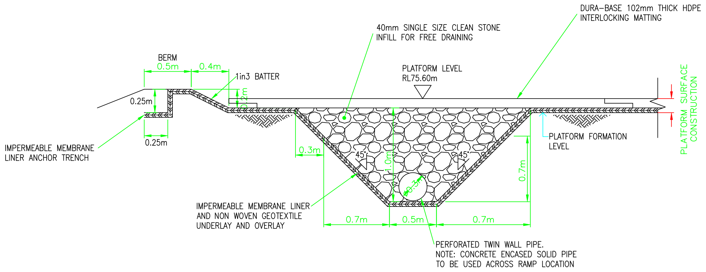
INDICATIVE SECTION THROUGH COVERED DITCH CONSTRUCTION DRILLING AND WELL TESTING PHASES (1:25 SCALE)
