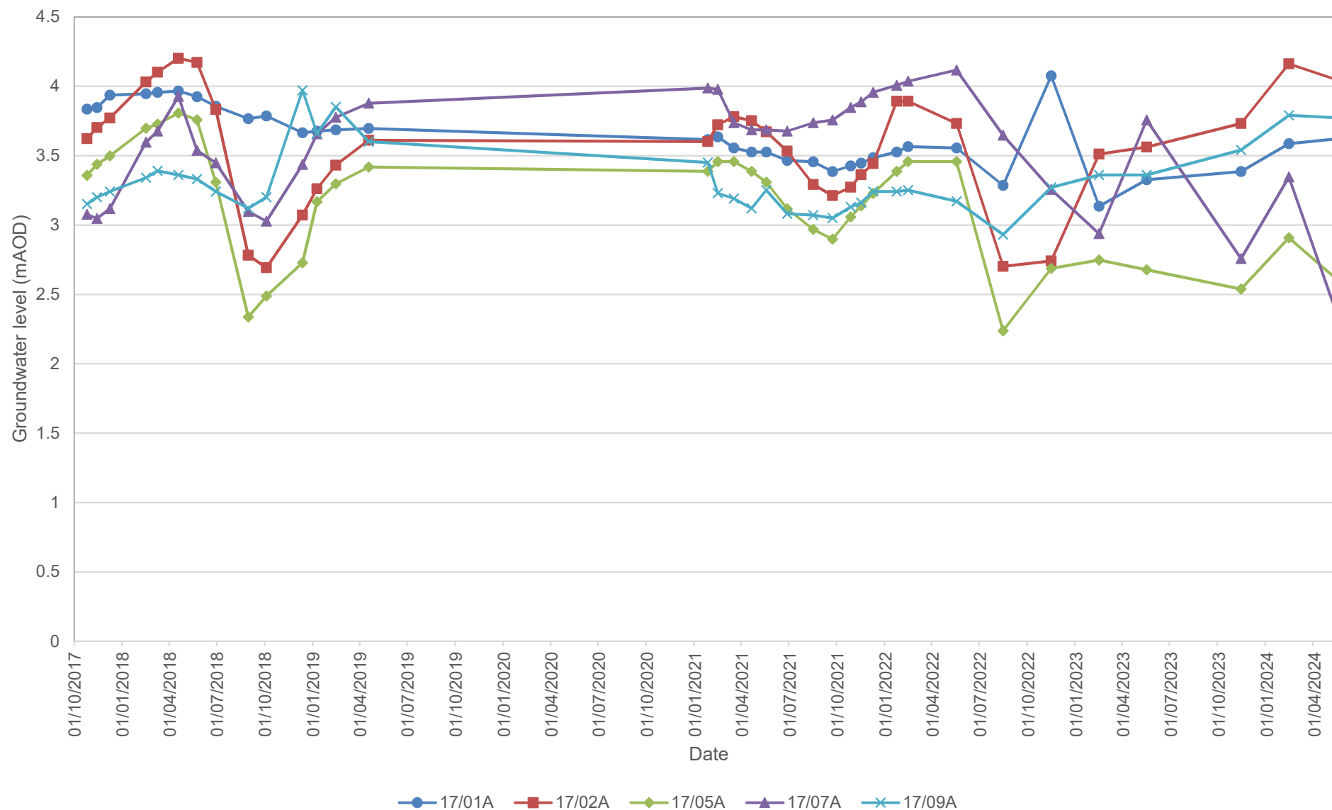
Figure ESSD 11 (UPDATED) - Groundwater levels recorded in the Sherwood Sandstone Group at groundwater monitoring boreholes at the Escrick site between October 2017 and May 2024
