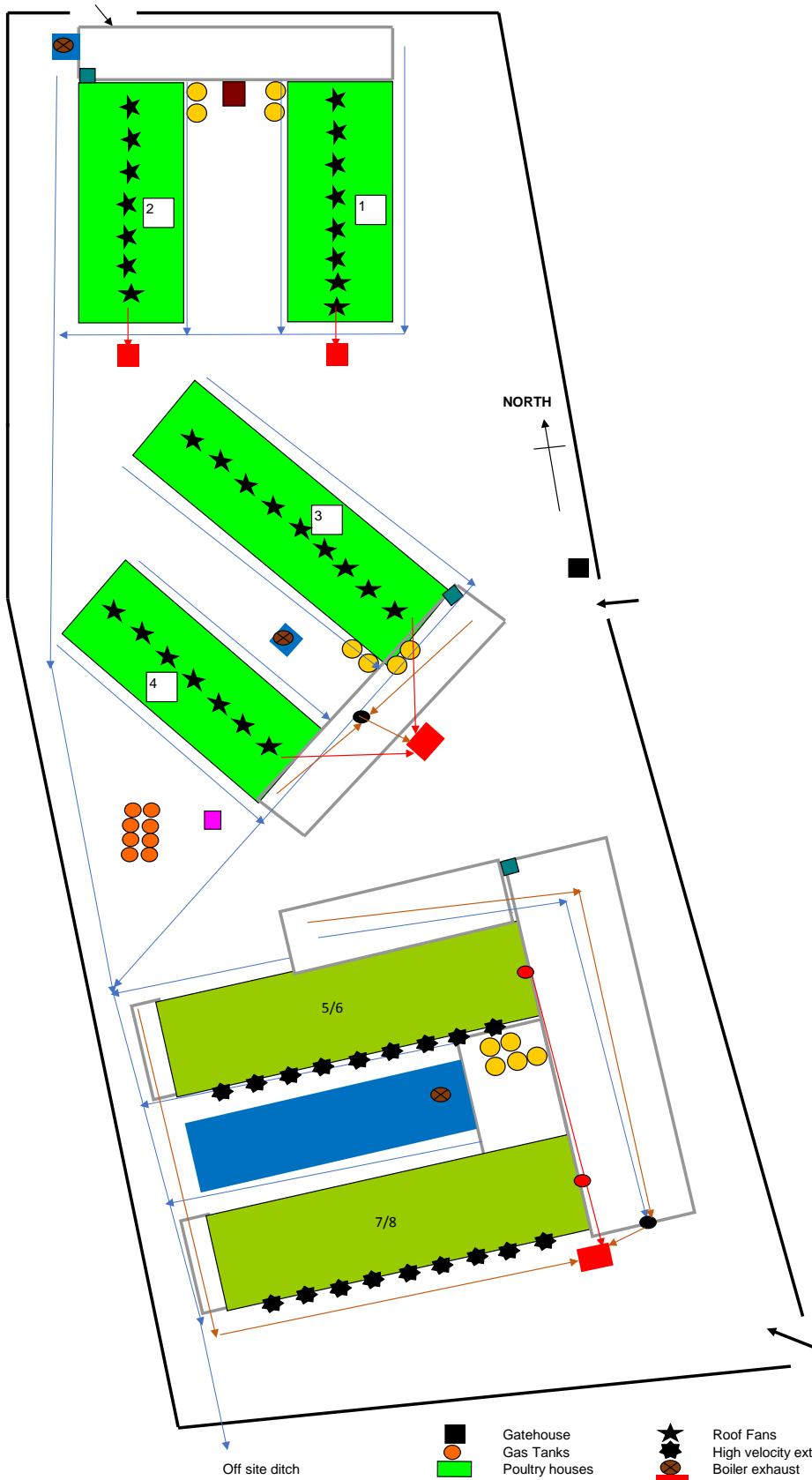
THORNGROVE LAYOUT PLAN
