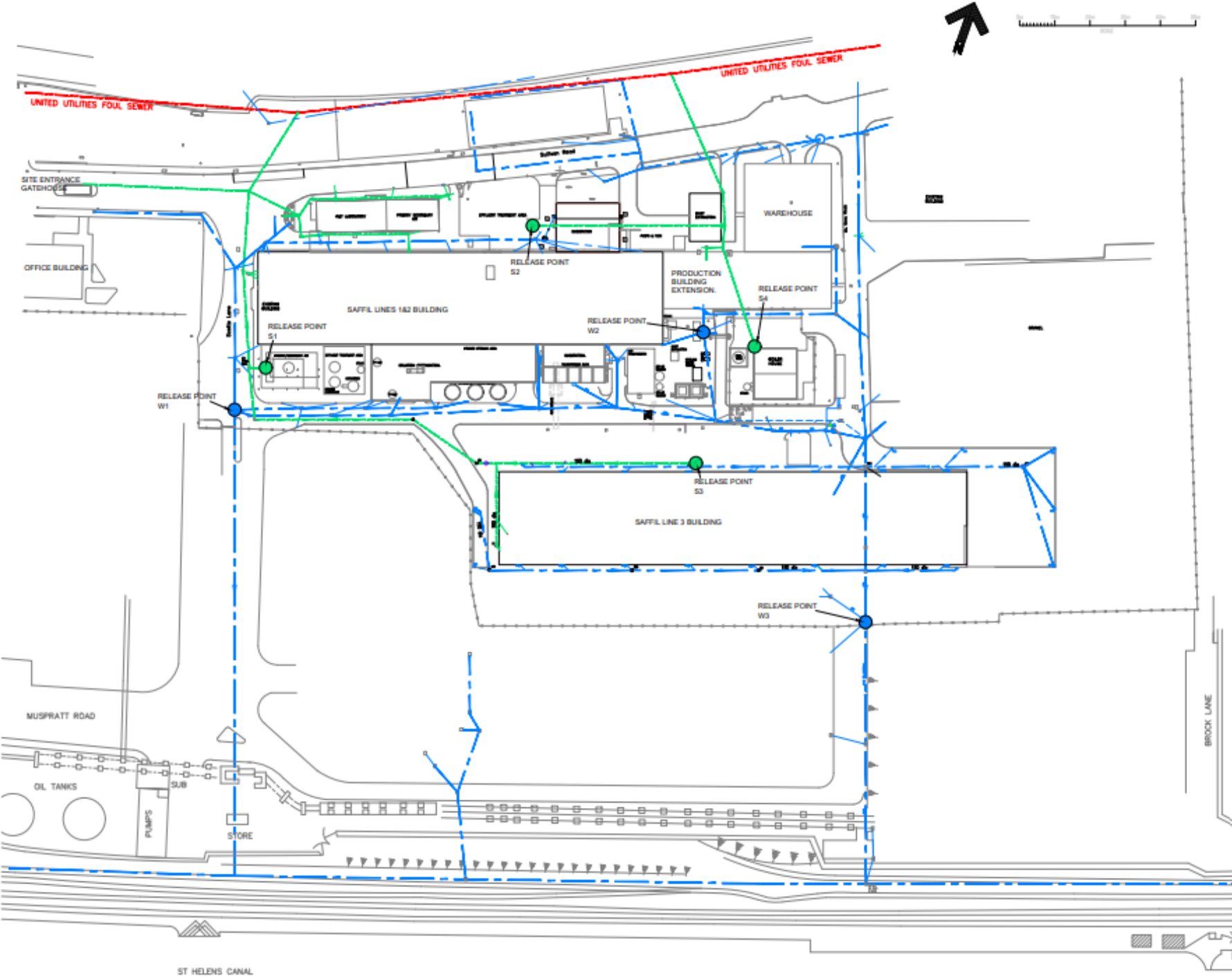
Widnes Site Drainage System Map (not to scale)
