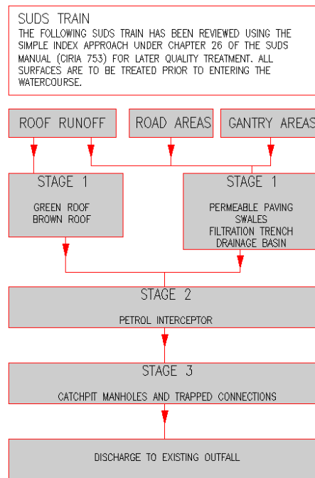
Figure 1 Table showing the proposed SuDS train for water quality treatment within the drainage strategy
