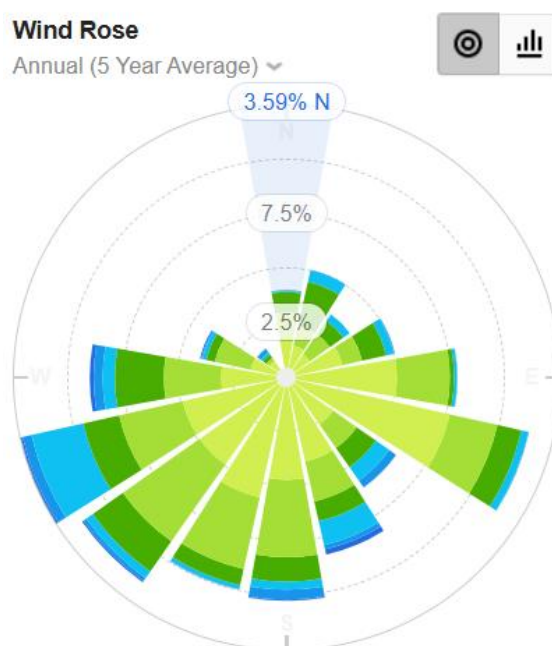
Wind rose Yeovilton observing station for the last five year
