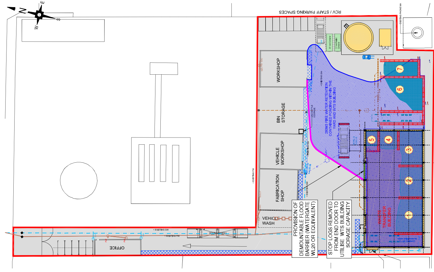
SCENARIO 2 - FIRE IN EXTERNAL STORAGE BAYS
