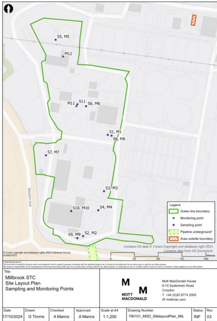
Figure 3: Layout and emissions on the Millbrook STC
