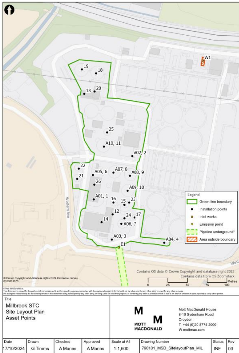
Figure 2: Layout and emissions on the Millbrook STC
