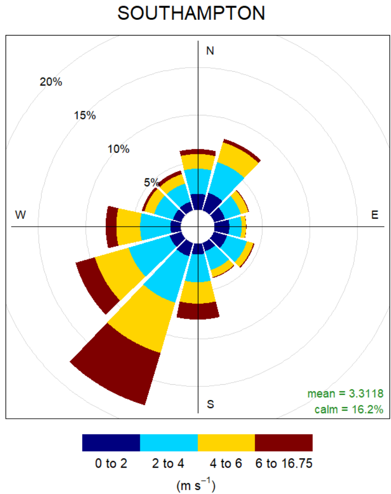
Figure 6: Average wind rose for Southampton meteorological site 2019- 2023
