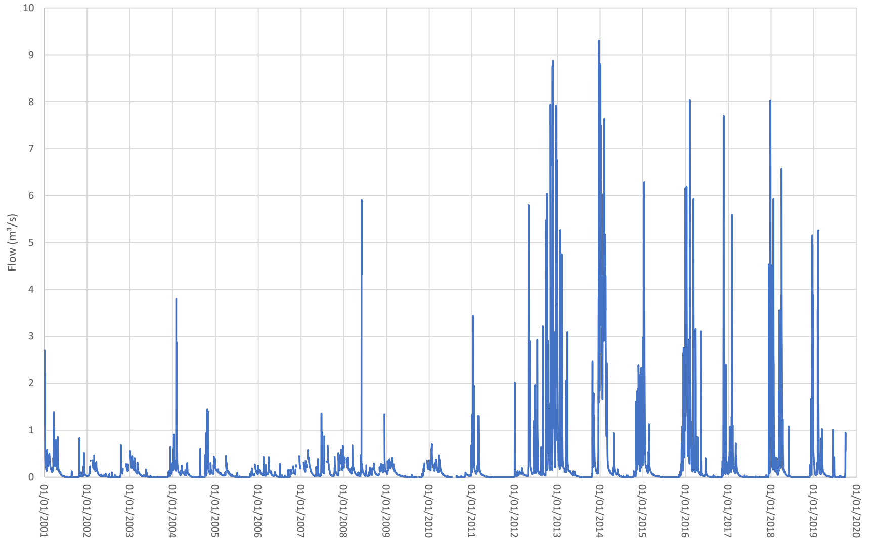
Marston Meysey Brook flow at Whetstone Bridge
