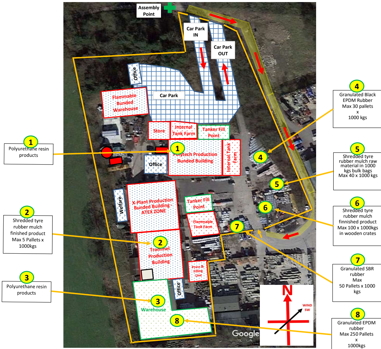
HS041 - Site Plans - Resin & Rubber Storage - A1
