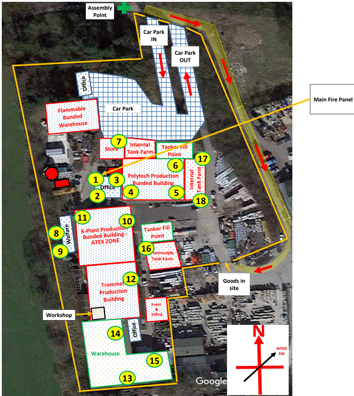
HS037 - Site Plans - Fire Alarm Call Points - A1
