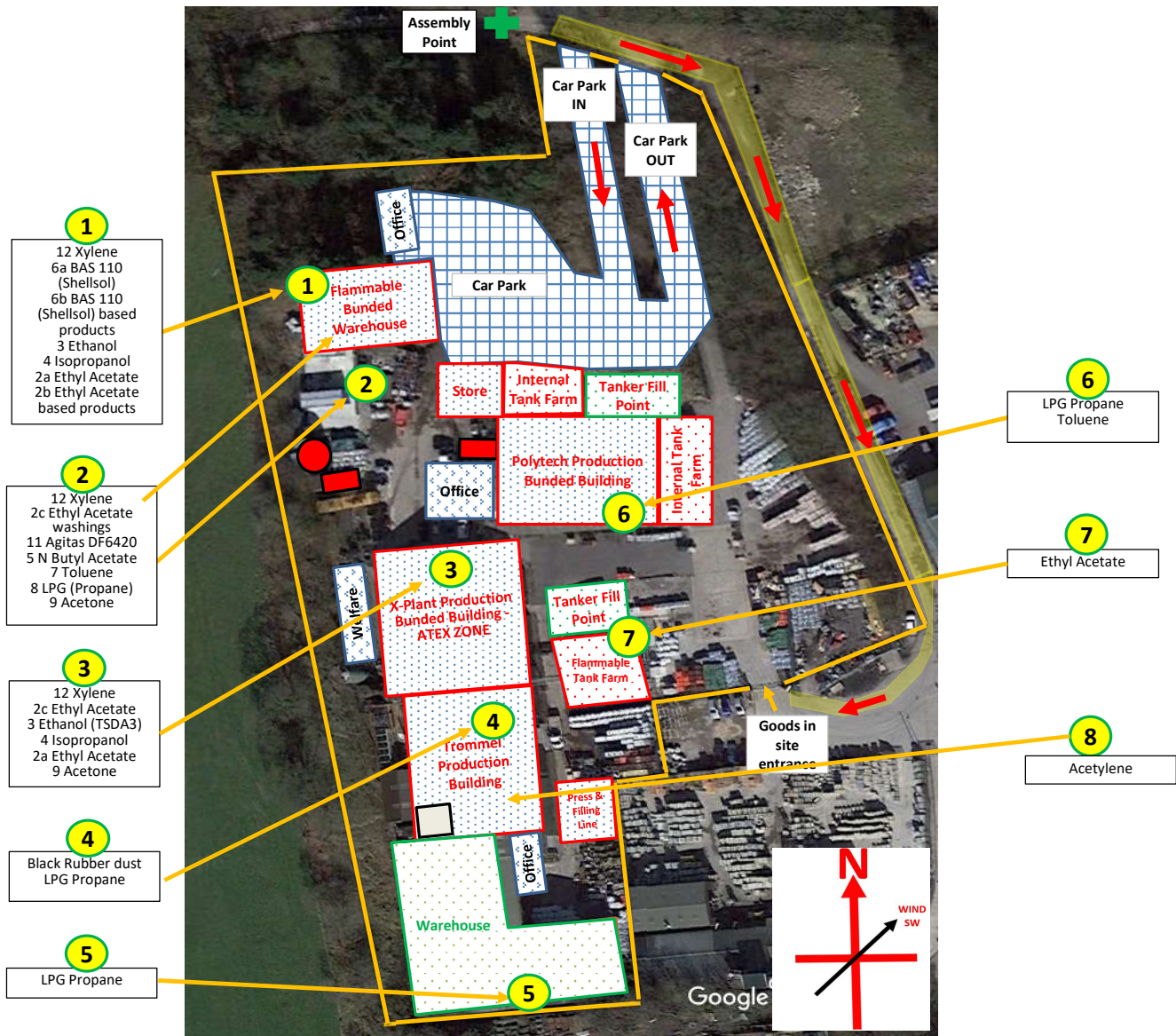
HS042 - Site Plans - DSEAR - A2
