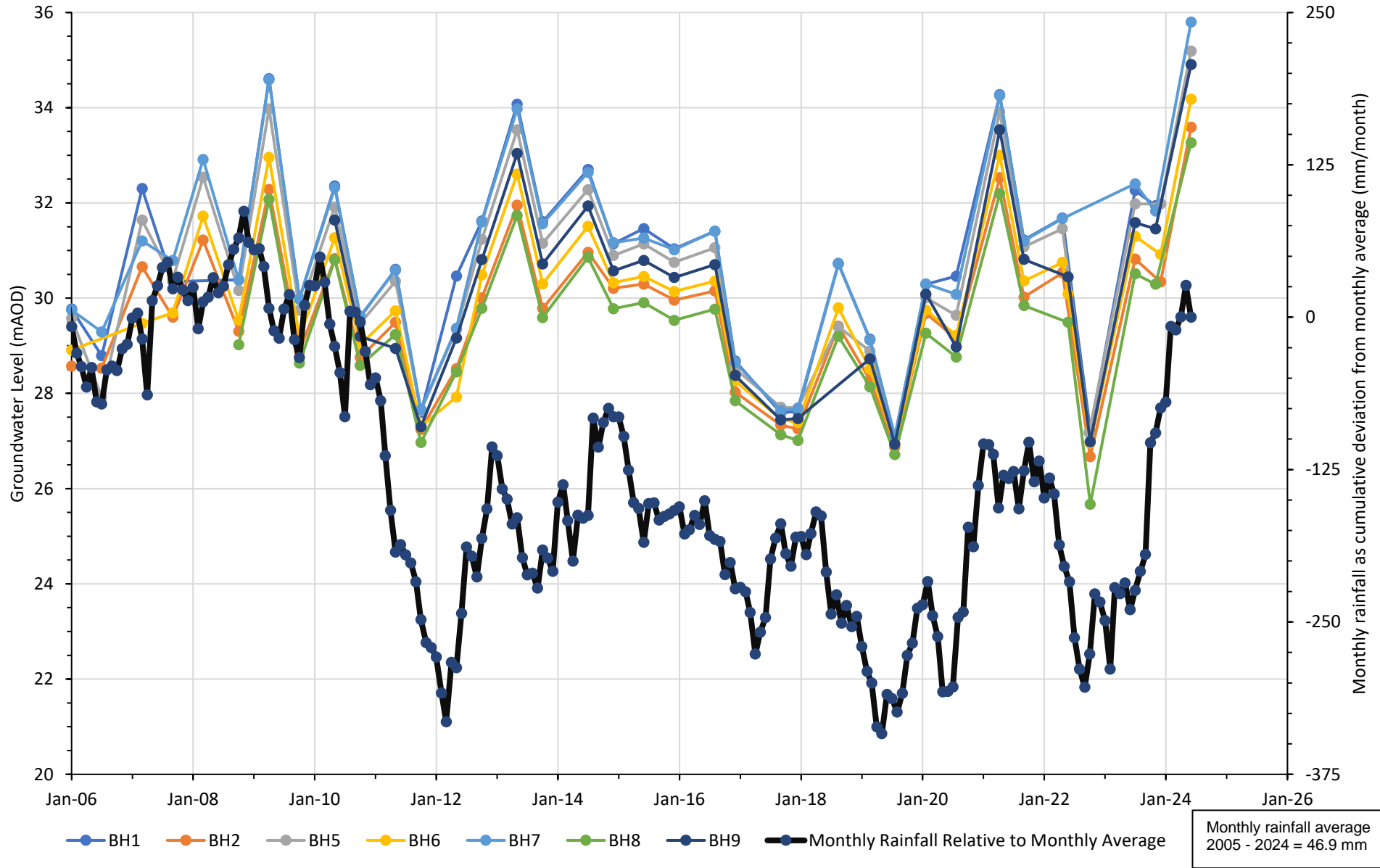
Royston Site: Groundwater Hydrographs and Rainfall
