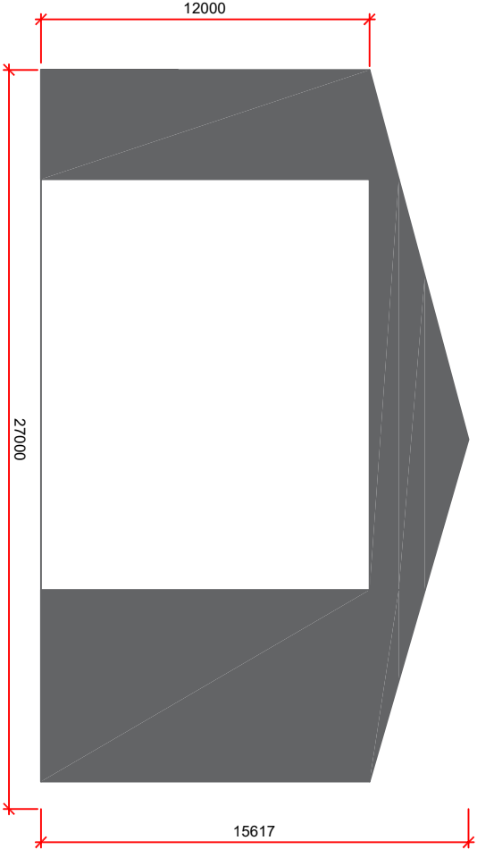
South Elevation
