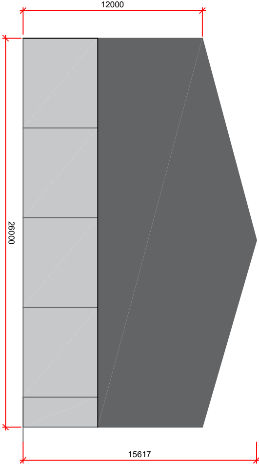
North Elevation
