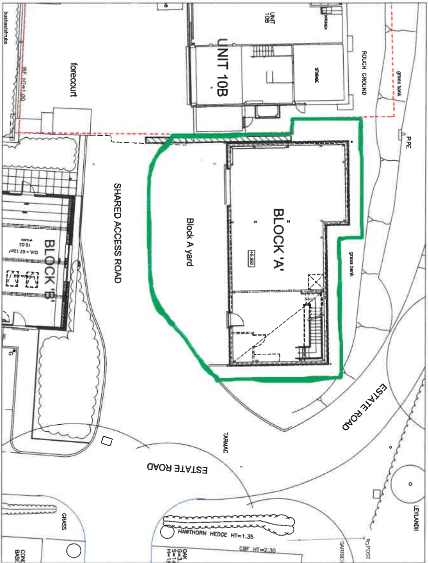
GROUND FLOOR PLAN 1:200 @ A3
