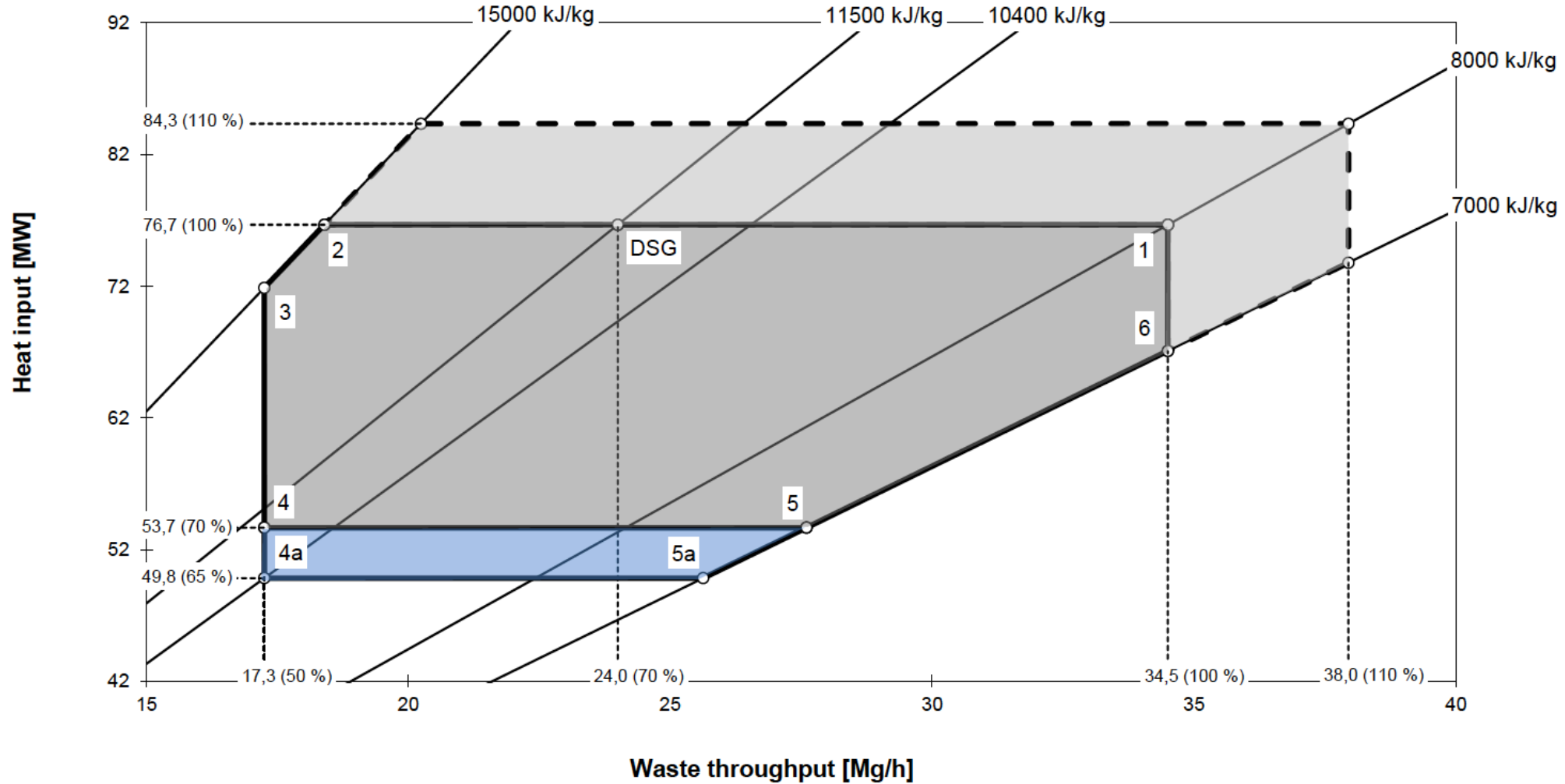
Wealden Works 3Rs Facility – Firing Diagram
