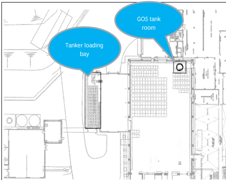
Figure 4-14 – GOS Bulk Tanker Loading Process
