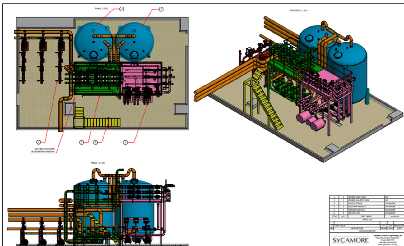
Figure 4-4 – New CIP Room Equipment Layout (CIP Set 7)
