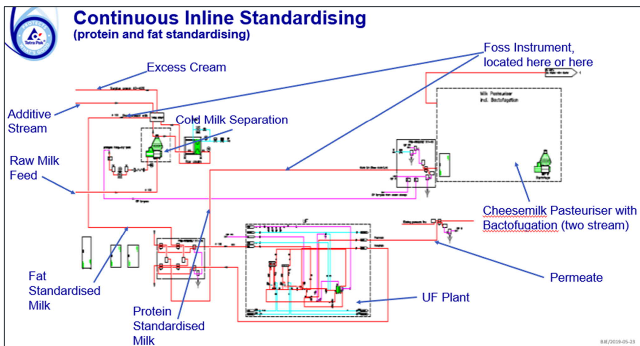
Figure 4-10 – Process Flow Diagram Showing Proten and Fat Standardisation
