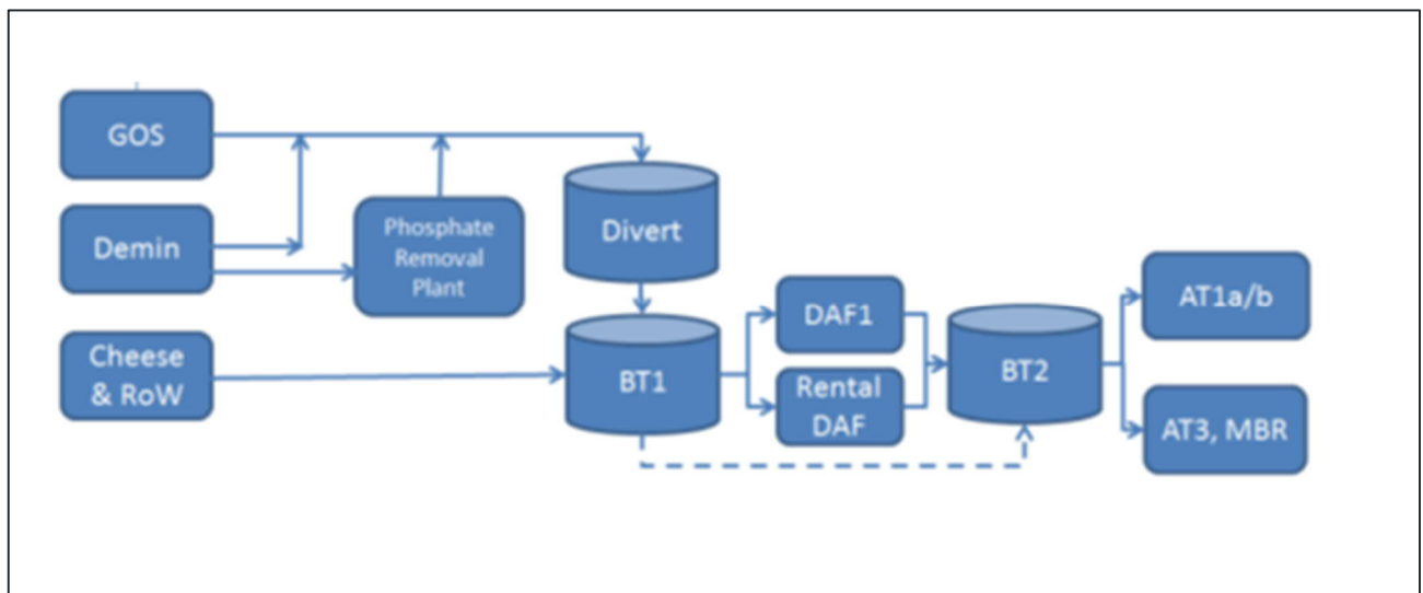
Figure 4-18 – Summary Flow Diagram of Effluent Configuration entering the WPF March 2017 to December 2017
