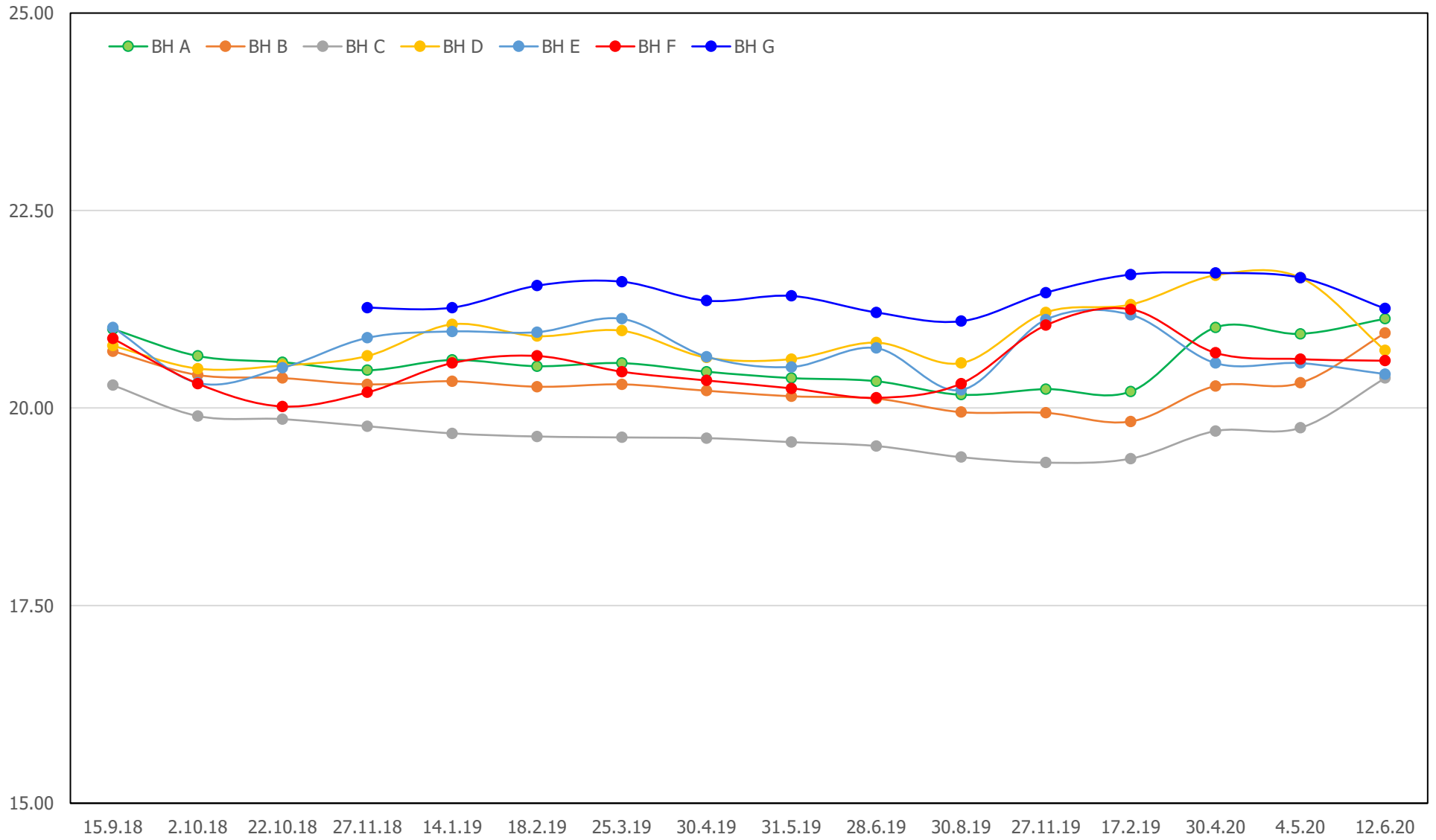
Crimplesham Groundwater Levels (mAOD)
