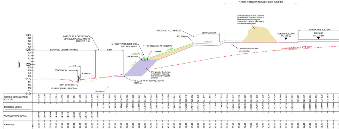
PLOT 1 - NORTH 03 - LONGSECTION SCALE: H 1:200,V 1:200, DATUM: 110.000 Remediation Profile
