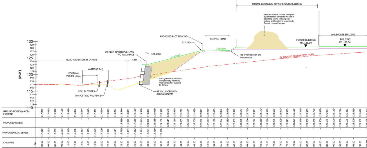
PLOT 1 - NORTH 04 - LONGSECTION SCALE: H 1:200,V 1:200, DATUM: 110.000 Remediation Profile
