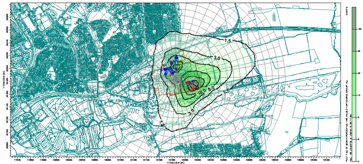
Figure 10: Great Billing WRC 98%ile hourly means odour contour map (year 2018). Zoom radius 1200m.
