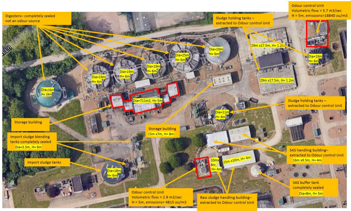
Figure 8: Great Billing STC – Details of the buildings, covered tanks, and odour sources in treatment site permitting area.
