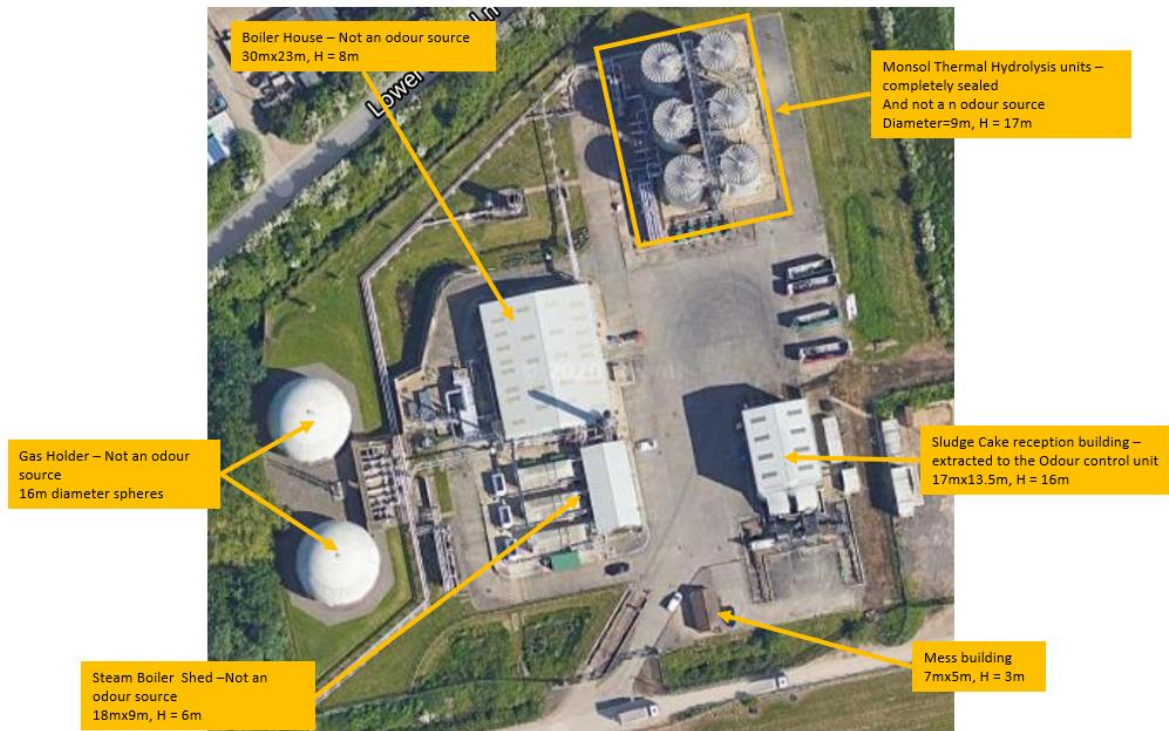
Figure 7: Great Billing STC – Details of the buildings, covered tanks, and odour sources in Monsol Thermal Hydrolysis plant permitting area.
