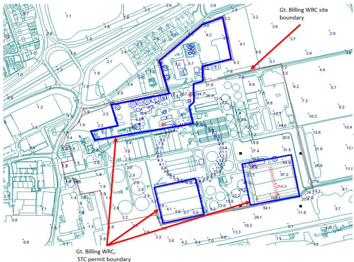
Figure 11: Great Billing STC 98%ile hourly means odour concentrations (year 2019). Around WRC and permit boundary
