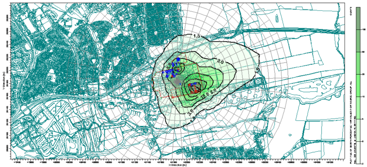
Figure 12: Great Billing STC 98%ile hourly means odour contour map (year 2020). Zoom radius 1200m.
