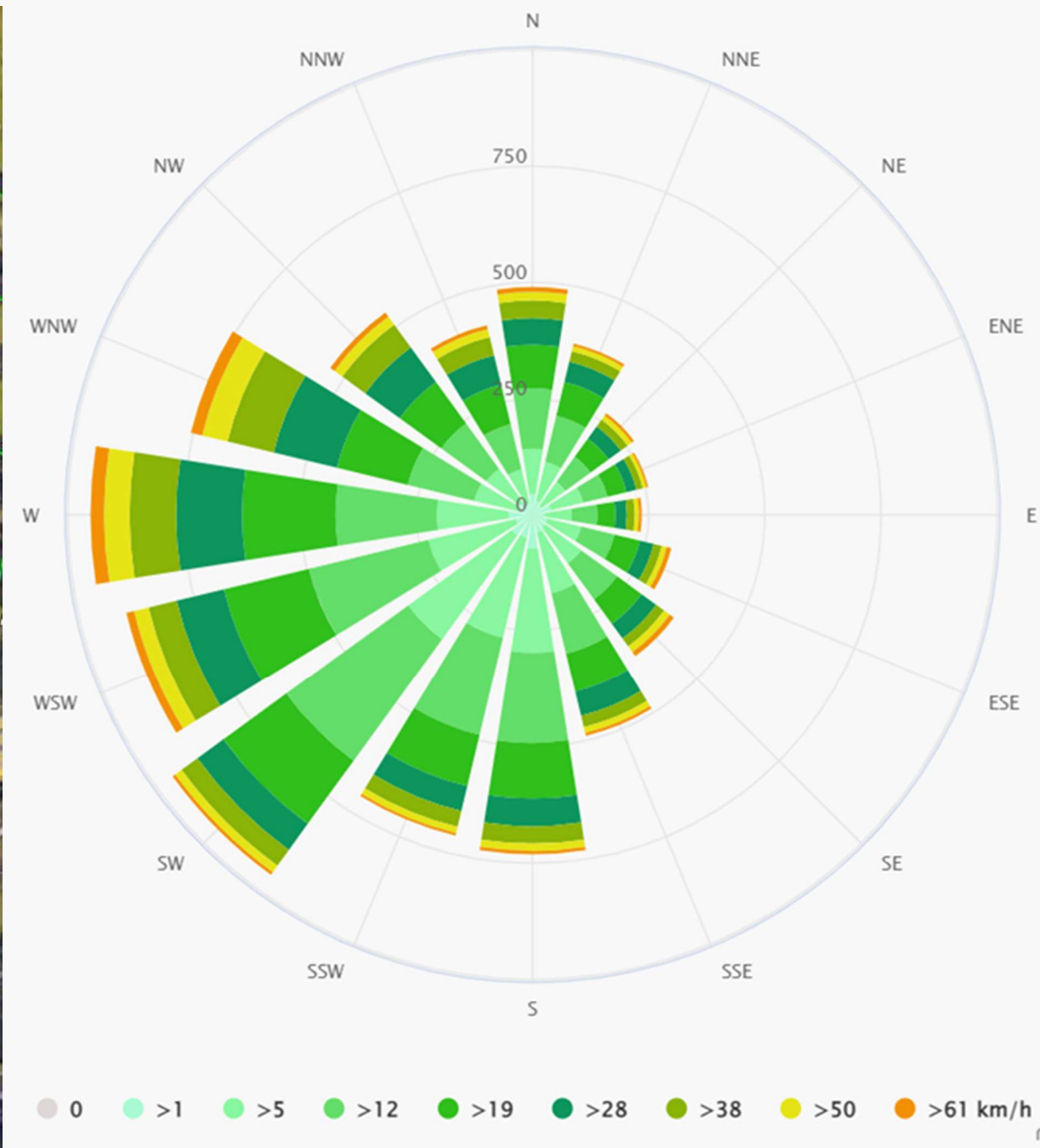
Aylesford Wind Rose: Source Meteoblue
