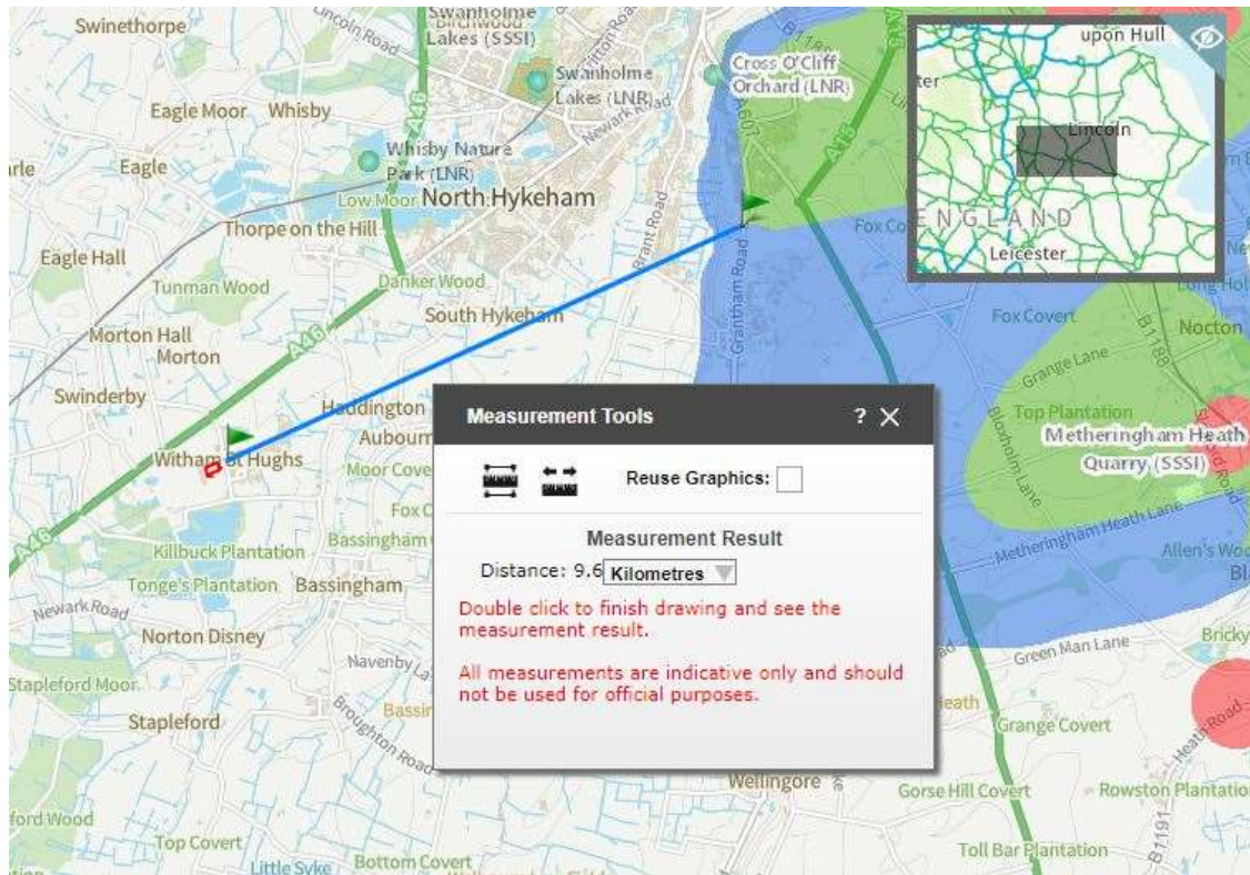
Figure 2 - Nearest groundwater source protection zones 1 & 2
