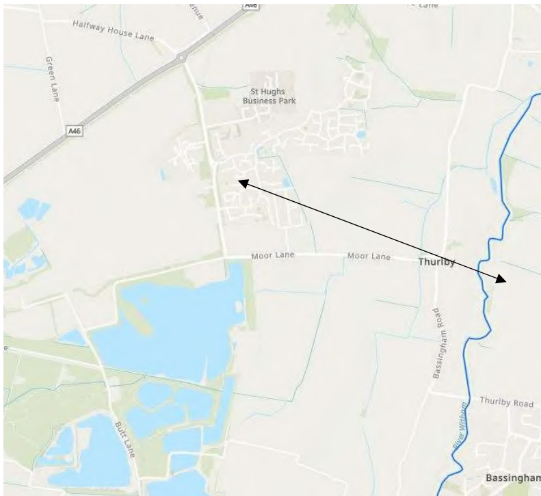
Figure 3 - Water Framework Directive Rivers Map
