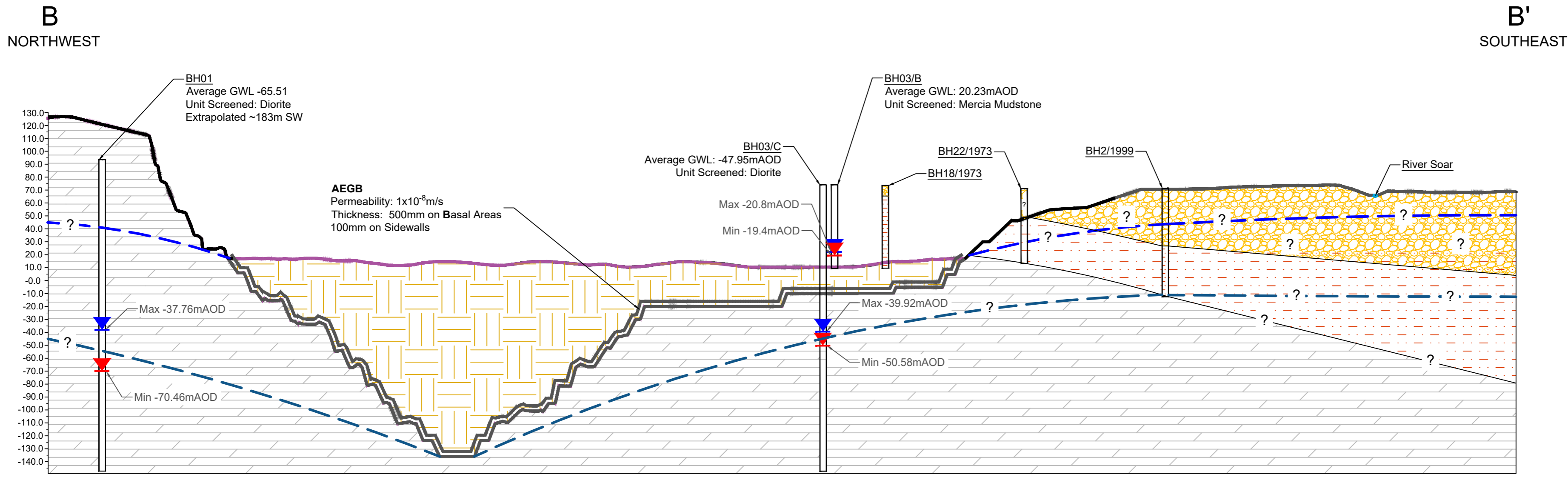
Section B-B' Scale - 1:2,500
