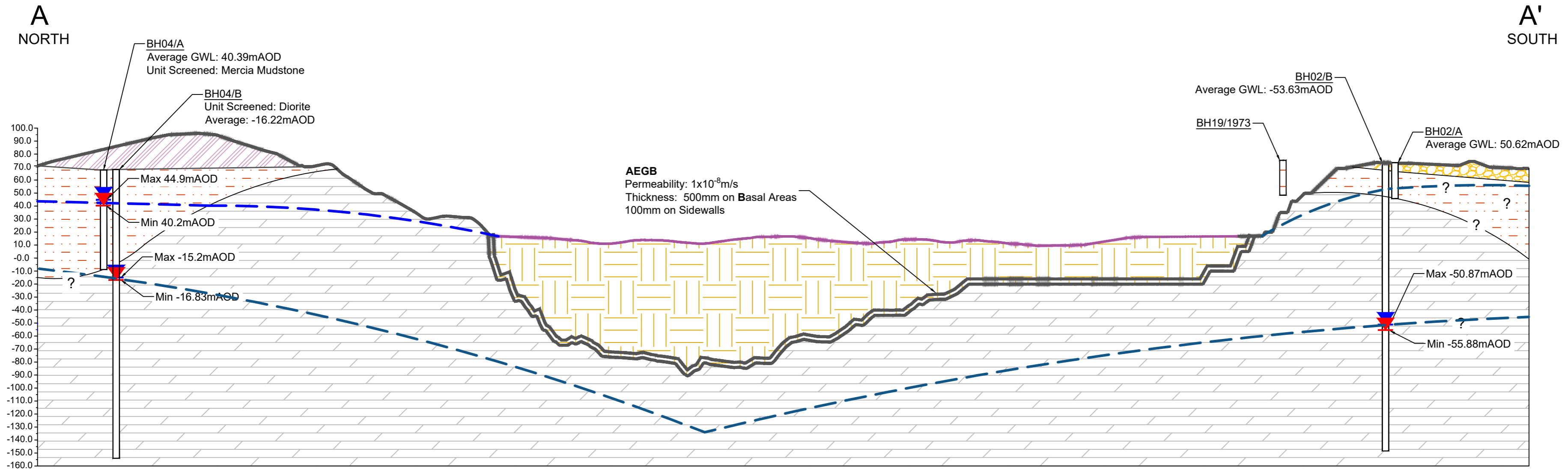
Section A-A' Scale - 1:2,500
