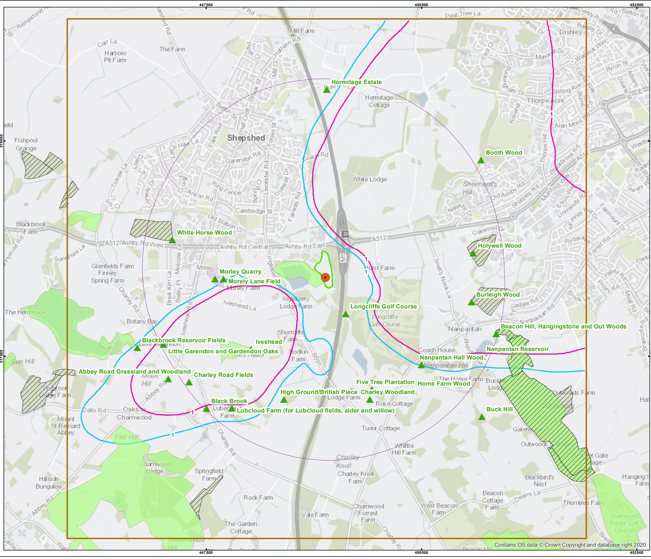
Figure 13 - Ecological receptors - annual mean oxides of nitrogen
