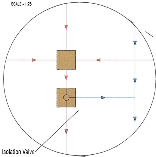
DIRTY/STORM WATER ISOLATION VALVE ARRANGEMENT
