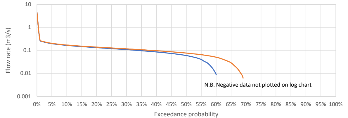
G1 Flow Duration Curve
