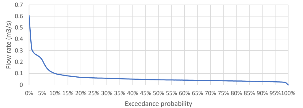
G4 Flow Duration Curve
