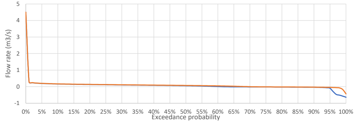
G1 Flow Duration Curve
