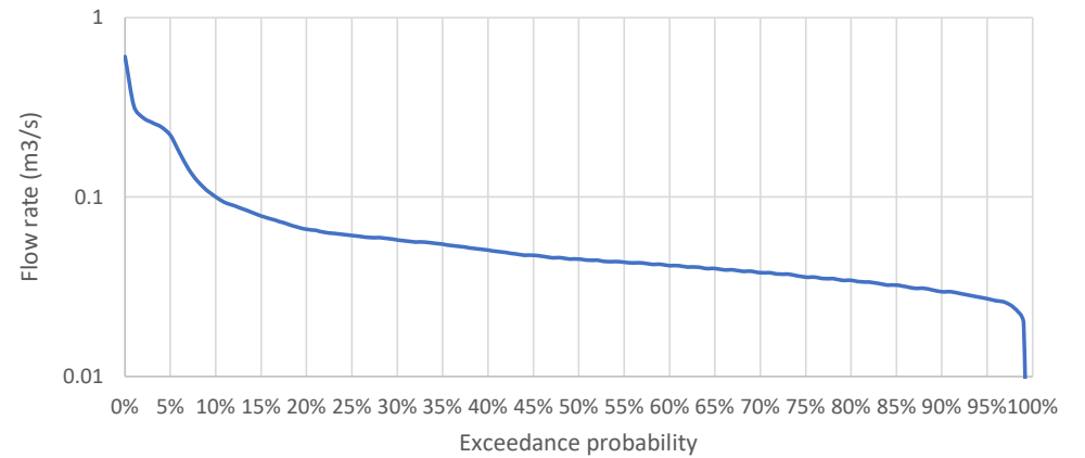
G4 Flow Duration Curve
