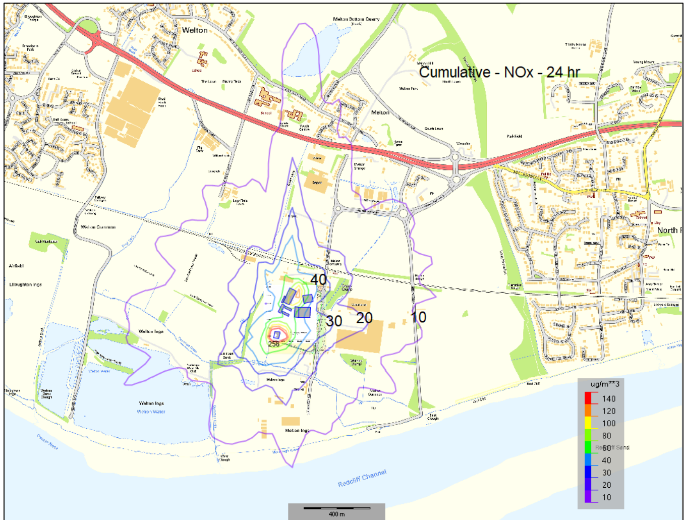
Figure 8-4. Predicted Ground level Short-Term (24 hr) NO x Concentrations (PC) for the Cumulative Assessment – Including Emissions from Eco-Power Boilers, Transwaste Kalvis Boilers and ERF (2018 Met Data)
