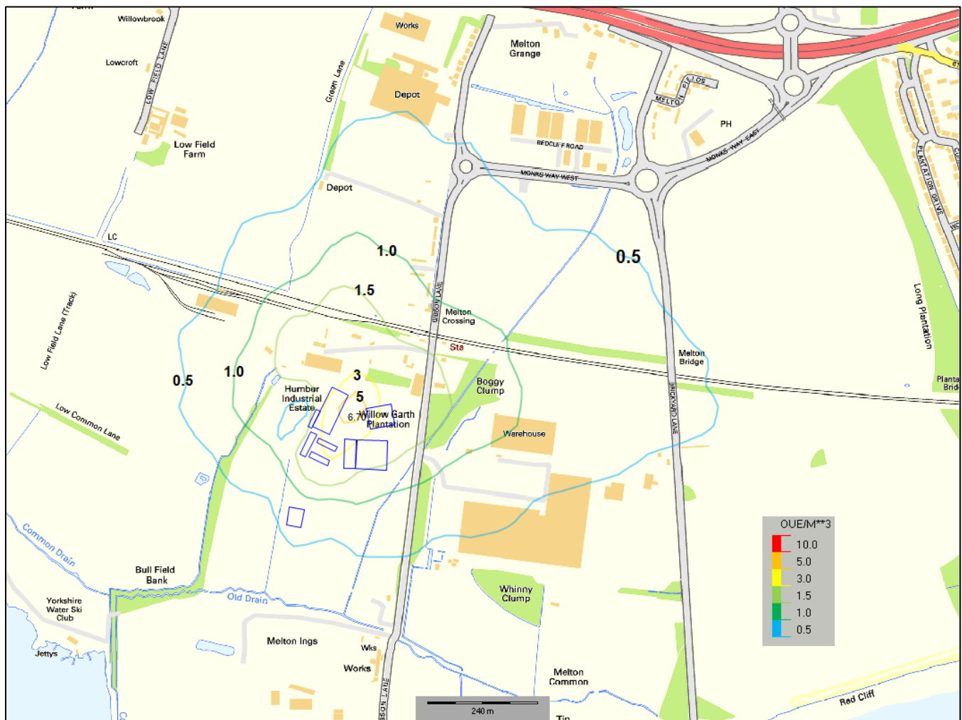
Figure 9-2. Predicted the 98 th percentile Short-Term (Hourly) Concentrations of Odour
