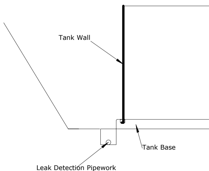
Cross Section Through Tank - 1:75
