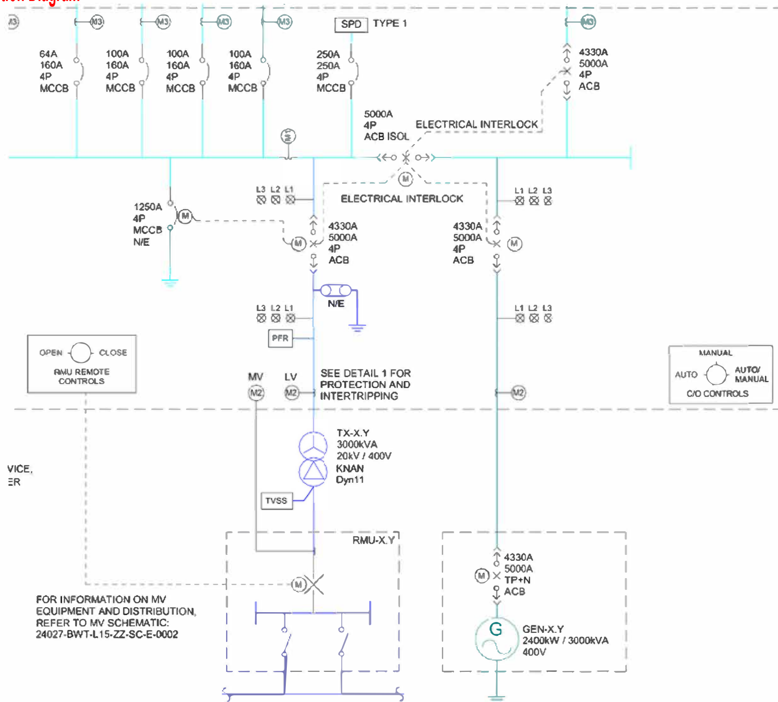
Figure B5 - Grid Connection Diagram
