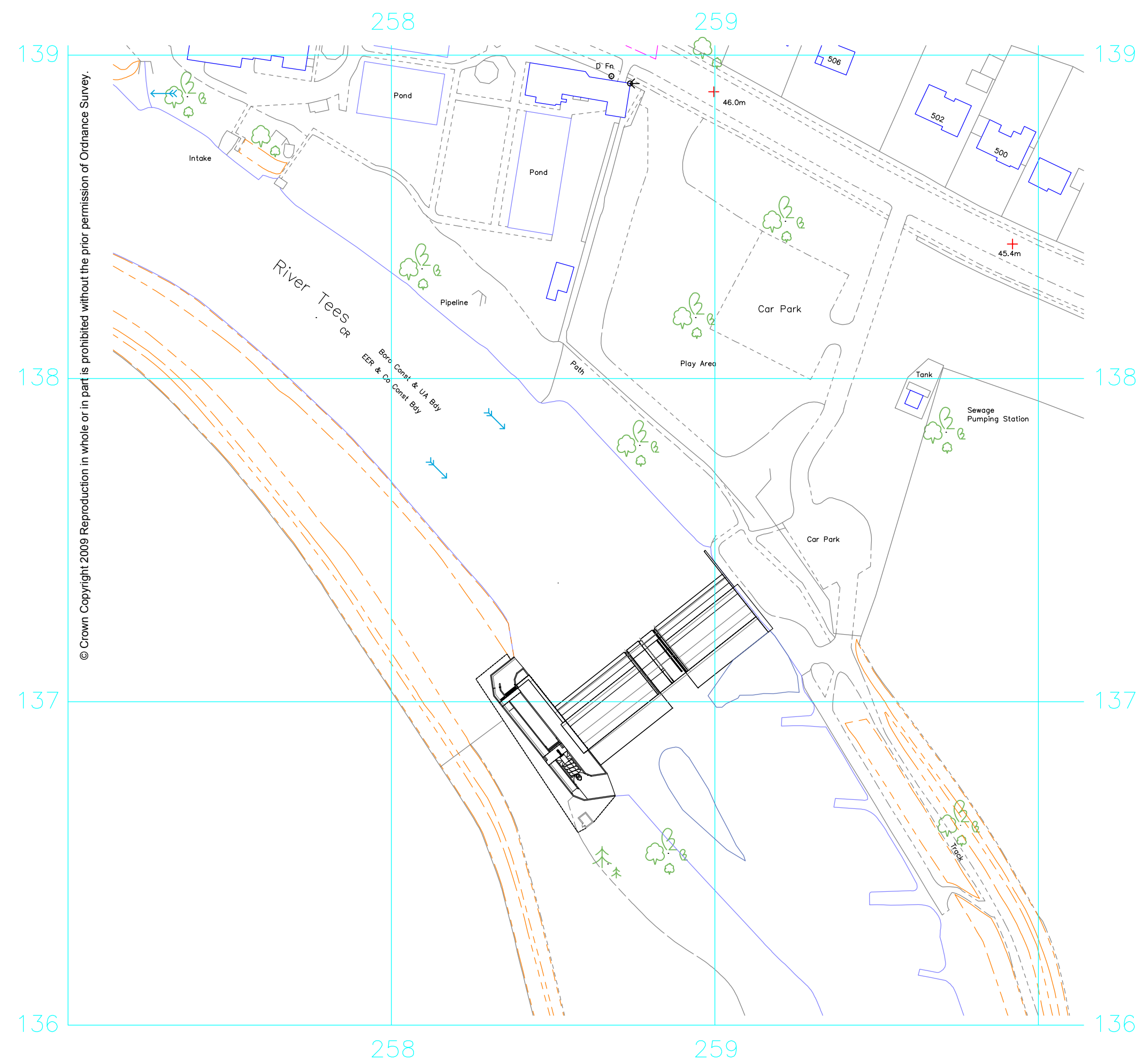
BLOCK PLAN: PROPOSED HYDRO PLANT (Scale 1:1250)
