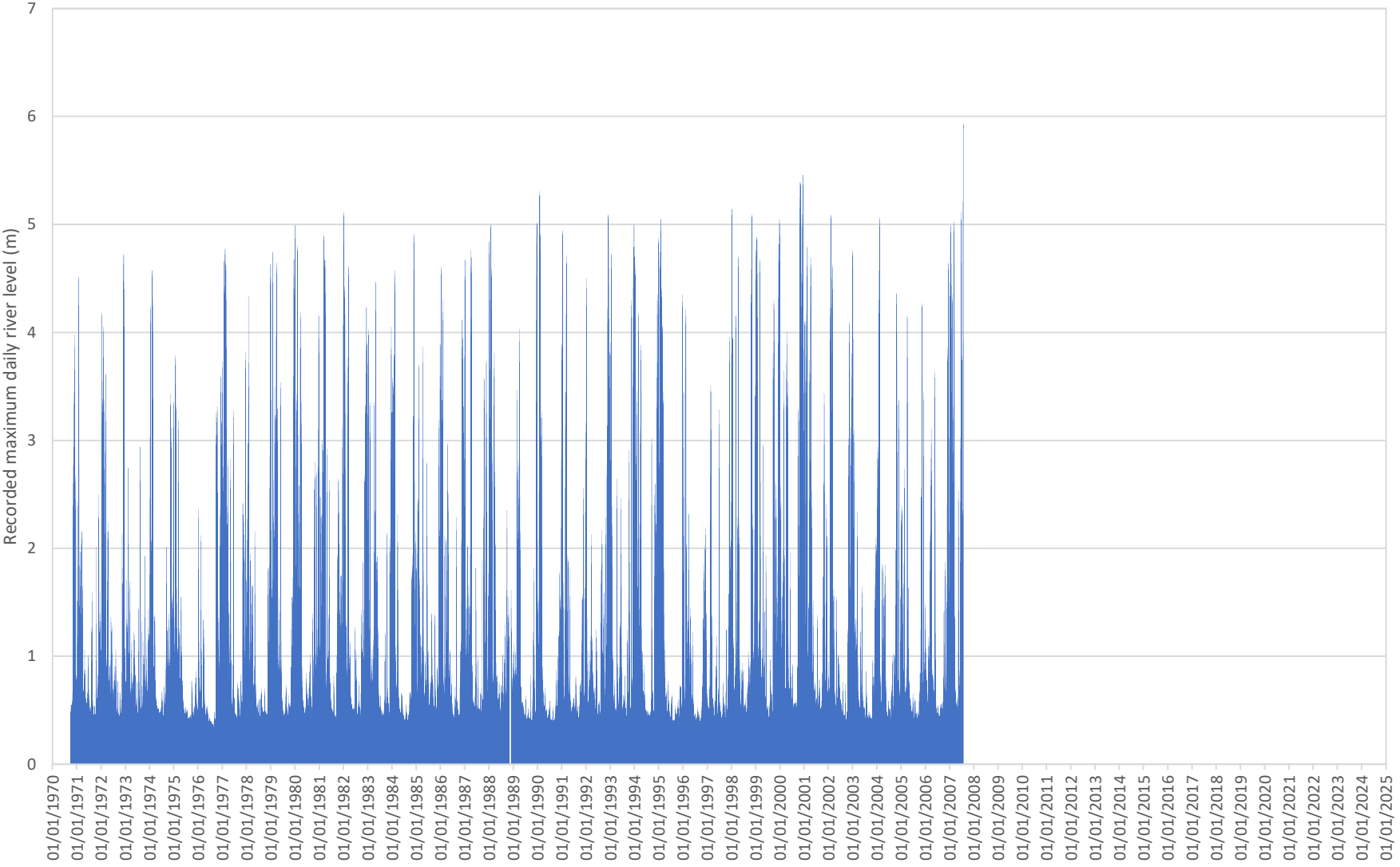
River Severn at Saxons Lode (Station Ref: 54032) - Recorded Maximum Daily River Levels
