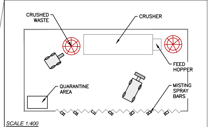
INSET A: WASTE STORAGE & PROCESSING BUILDING FLOOR PLAN
