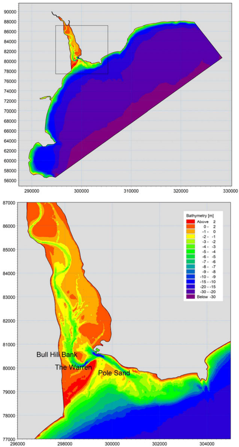
Figure 2-3. Model bathymetry
