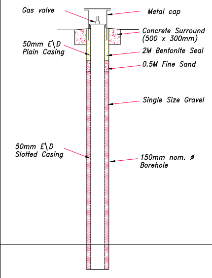
SECTION THROUGH GAS MONITORING BOREHOLE GAS MONITORING POINT
