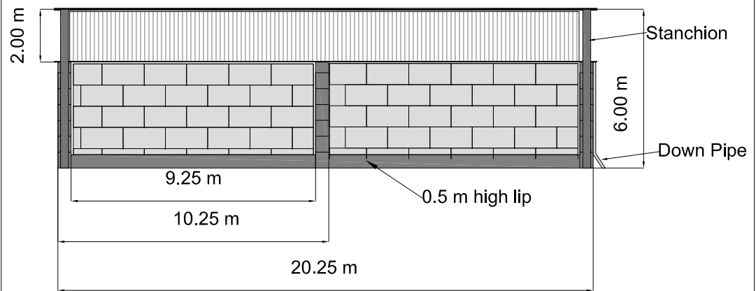
Area 4 Enclosure Front View
