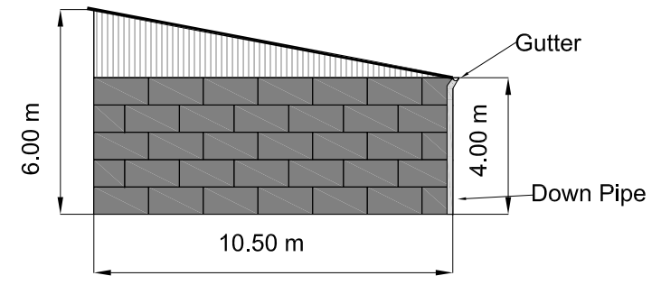
Area 4 Enclosure Side View
