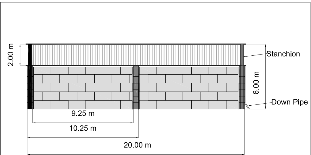
Area 2 Enclosure Front View
