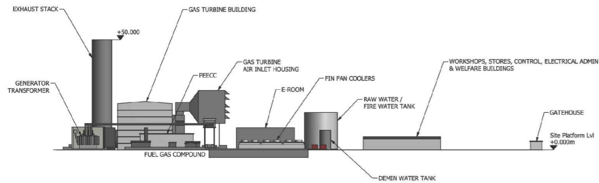
SOUTH ELEVATION
